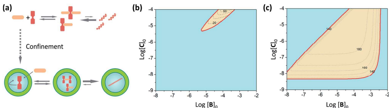
Fig. 7 (a) Schematic illustration of the effect of confinement of C . (b) Plot showing the range of concentration of C and B at which the double stranded polymer is the dominant species ( i.e. , more than 50% of C involved in the polymer) (red area) for non-confined C . The dashed lines show the average number of repeats of the polymer formed in increments of 10 repeats. (c) Same as (b) for confined C . In all cases the binding constants used are those in Table 1, with K_1 averaged between the non-confined and confined values, and the total concentration of C in the cavity of the vesicles is 1 mM.
