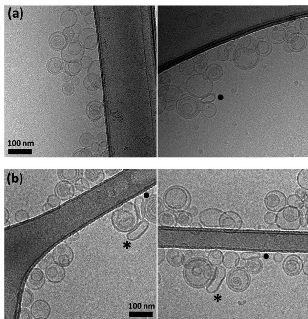
Fig. 8 (a) Detail of a cryo-TEM image of a sample of vesicle-confined C ( [C]_0 = 1.8 \mu\text{M} and [C]_a = 1 \text{ mM} ). (b) Detail of a cryo-TEM image of a sample vesicle-confined C in the presence of B ( [C]_0 = 1.8 \mu\text{M} , [C]_a = 1 \text{ mM} , [B]_0 = 32 \mu\text{M} ). The symbol (•) is used to highlight vesicles that appear flattened by the physical constrains imposed by the carbon film support and surrounding vesicles, while (*) is used to highlight vesicles that appear flattened without apparent physical constrains.
