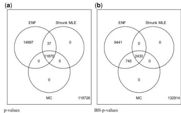
Fig. 7. Amount of significant edges related to lung samples' expression in M.musculus . Analysis of M.musculus RNA-seq expression data from lung samples (Steed et al., 2017). The estimator produces an optimal shrinkage \lambda \approx 0.11 . Three methods are compared at \alpha = 0.10 : ENF, Shrunk MLE and MC (with 40 iterations). Panel (a) Venn diagram of significant partial correlations (i.e. edges in the GGM) recovered by each method with un-adjusted P -values. Panel (b) Venn diagram of significant partial correlations recovered by each method with BH-adjusted P -values
