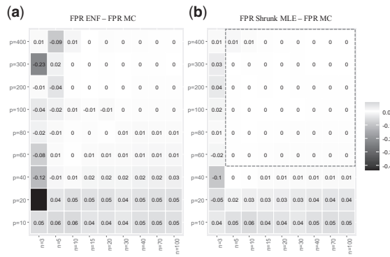
Fig. 4. FPR cross-comparison. This figure shows a heatmap for the difference in FPR under H_0 : no partial correlation with respect to the gold standard (MC). The number of variables p range from 10 to 400, and the sample size n from 3 to 100. Panel (a) shows the heatmap for the FPR for ENF minus the FPR for MC, averaged over 10 simulations (rounded to two decimals). Panel (b) show the respective results for Shrunk MLE. The test is carried out at \alpha = 0.05 with a shrinkage value fixed to \lambda = 0.3 . The color scale represents the FPR differences in the p - n grid, where the larger the FPR difference the darker is the corresponding grid cell. In general, Shrunk MLE outperforms ENF, and it is in close agreement with MC for p > 40 and n > 10
