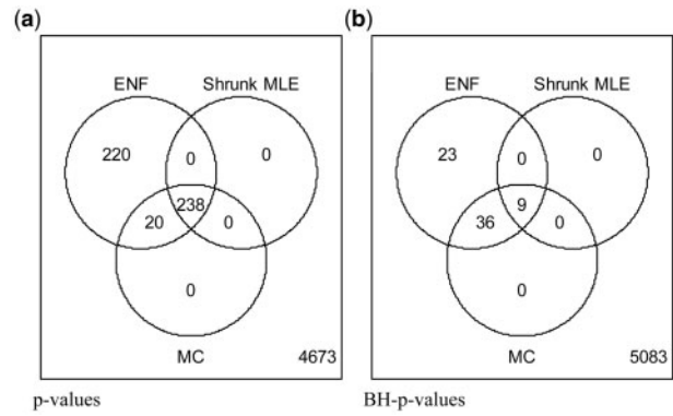
Fig. 6. Amount of significant edges related to the induced expression of SOD in E.coli . Analysis of E.coli gene microarray expression data upon response to induced SOD expression. The dataset includes 102 genes (Schmidt-Heck et al., 2004). The estimator produces an optimal shrinkage \lambda = 0.18 . Three methods are compared at \alpha = 0.05 : ENF, Shrunk MLE, MC with 40 iterations. Panel (a) Venn diagram of significant partial correlations (i.e. edges in the GGM) recovered by each method with un-adjusted P -values. Panel (b) Venn diagram of significant partial correlations recovered by each method with BH-adjusted P -values
