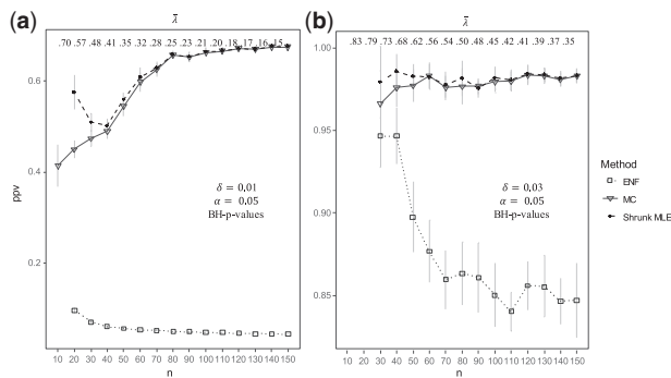
Fig. 5. Positive predictive value. This figure shows the PPV ( PPV = TP/P ) obtained with different sample sizes. The inference is carried out from simulated data for p = 100 with n ranging from 10 to 150 in steps of size 10, tested at \alpha = 0.05 . The Panels (a) and (b) show the PPV using Benjamini-Hochberg (BH)-adjusted P -values for multiple testing with \delta = 0.01 (or 49 correlations) and \delta = 0.03 (or 148 correlations). Three approaches are compared: ENF (dot with dashed line), Shrunk MLE (square with dotted line), and MC with 15 iterations (triangle with continuous line). Symbols (and bars) represent the average ( \pm 2 SEs) over 25 repeated simulations. The upper horizontal axis shows the average shrinkage intensity \bar{\lambda} rounded to two digits
