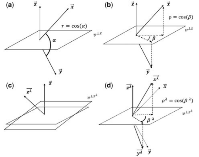
Fig. 1. Geometry of the partial correlation. The vectors \vec{x} , \vec{y} and \vec{z} represent the random variables X , Y and Z in subject space. In Panel (a), the correlation r between X and Y is the cosine of \alpha . In Panel (b), the partial correlation between X and Y can be interpreted as the cosine of the angle \beta . That is the cosine between the projection of \vec{x} and \vec{y} onto a plane orthogonal to \vec{z} . The shrinkage effect consists in that the vectors \vec{x} , \vec{y} and \vec{z} are transformed to \vec{x}^\lambda , \vec{y}^\lambda and \vec{z}^\lambda such that their lengths remain 1, and only the angles between each other change. In other words, the transformed vectors become less correlated. In Panel (c), the geometrical effect of the shrinkage consists in changing the projection plane v^\perp z to v^\perp z^\lambda . In Panel (d), the ‘shrunk’ partial correlation \rho^\lambda between X and Y is the cosine of the angle \beta^\lambda . That is the cosine between the projections of \vec{x}^\lambda and \vec{y}^\lambda onto v^\perp z^\lambda .
