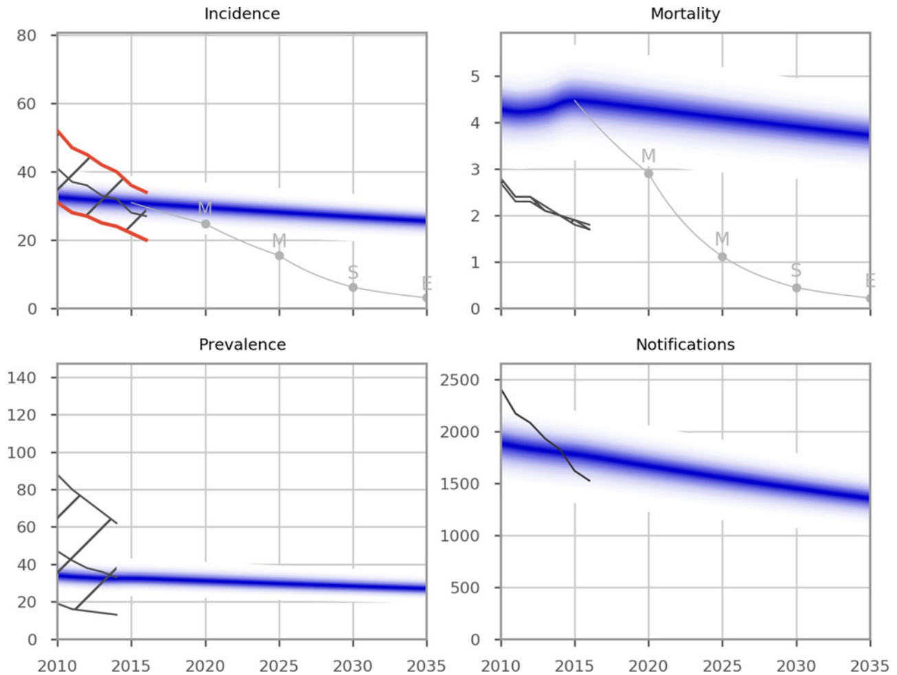
Fig. 1. Epidemiological calibration results. The blue shaded areas represent model estimates. The black lines and hatched areas are mean values and confidence limits, respectively, for indicator data from the WHO Global TB report (2016 and 2017). Data from the WHO Global TB Report 2017 were used for the years from 2000 to 2016. As the WHO Global TB Report 2017 did not report data prior to 2000, the WHO Global TB Report 2016 was used for data points for the years that were not included in the 2017 report (1990 to 1999). The red lines in the Incidence panel indicate the WHO incidence data points against which the model was calibrated. Grey lines represent the SDG targets for 2030, the End TB Strategy targets for 2035 and the interim milestones for 2020 and 2025. Units of all horizontal axes are calendar years and units of vertical axes are: incidence, per 100 000 per year; mortality, per 100 000 per year; prevalence per 100 000; notifications, absolute number.
