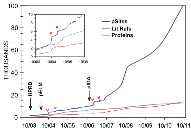
Figure 1. Informational content of PhosphoSite ® curated from the literature from its launch in 2003 through 2011. Phosphorylation sites (blue), proteins (red) and references (gray). The approximate dates that descriptions of three other resources were published are indicated by black arrows: HPRD (19), phospho.ELM (20) and PHOSIDA (21). Inflection points indicate the publication of large MS data sets; a few are marked with red arrowheads.
