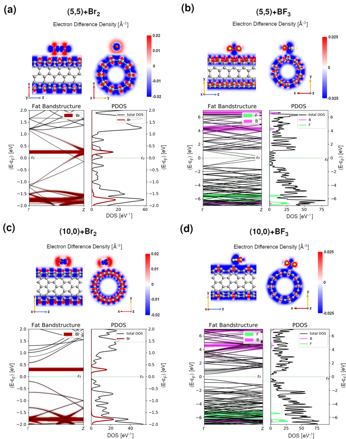
Figure 10. Computed electronic properties of (5,5) and (10,0) CNTs interacting with (a,c) Br 2 and (b,d) BF 3 molecules, respectively. (top panels) The electron different densities and (bottom left panels) fat band structures along \Gamma \rightarrow Z of the Brillouin zone together with the projected density of states on chosen atomic species (PDOS) (bottom right panels). Br atoms are depicted in red while B, F and C atoms are shown in pink, light green, and grey, respectively.
