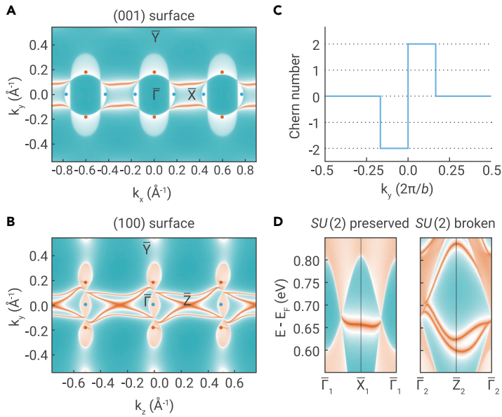
Figure 4. Protected topological surface states of flavor WSM CoNb 3 S 6 (A and B) Iso-energy surface states connect electron pockets and hole pockets, separately enclosing flavor Weyl points with opposite chirality on (001) and (100) surfaces of CoNb 3 S 6 . (C) The transition of Chern number defined on 2D slices in the Brillouin zone perpendicular to the y axis as a function of momentum k_y . (D) Chiral edge states of the 2D slice ( k_y = 0.1 (2\pi/b) ) with Chern number of 2. Doubly degenerate edge bands are found in SU(2) -preserved edge, while spin-polarized nondegenerate edge bands are found in SU(2) -broken edge. The notations are defined as \bar{\Gamma}_1 = \bar{\Gamma} + \bar{P} , \bar{X}_1 = \bar{X} + \bar{P} , \bar{\Gamma}_2 = \bar{\Gamma} + \bar{P} , and \bar{Z}_2 = \bar{Z} + \bar{P} , where \bar{P} = \frac{1}{2}(\bar{Y} - \bar{T}) .
