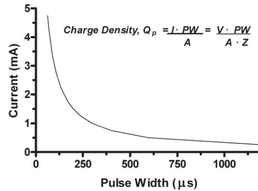
Figure 2. Plot of current vs. pulse width values yielding a charge density ( Q_p ) of 30 \mu\text{C}/\text{cm}^2/\text{phase} . For this study, DBS delivery was programmed in constant current mode. To determine initial DBS parameter settings of current (I) and pulse width (PW) that could be presumed not to cause tissue damage, a safety threshold curve was generated from PW and I combinations that yielded a charge density ( Q_p ) of 30 \mu\text{C}/\text{cm}^2/\text{phase} – a clinical reference value used as a conservative safety threshold for DBS applications. The equation insert in the graph was used to calculate corresponding PW values for a range of I values, with A=0.01 \text{ cm}^2 for the area of the electrode we used and Q_p=30 \mu\text{C}/\text{cm}^2/\text{phase} . Thus, any I and PW combinations to the left of the safety-threshold curve could initially be selected. doi:10.1371/journal.pone.0030672.g002
