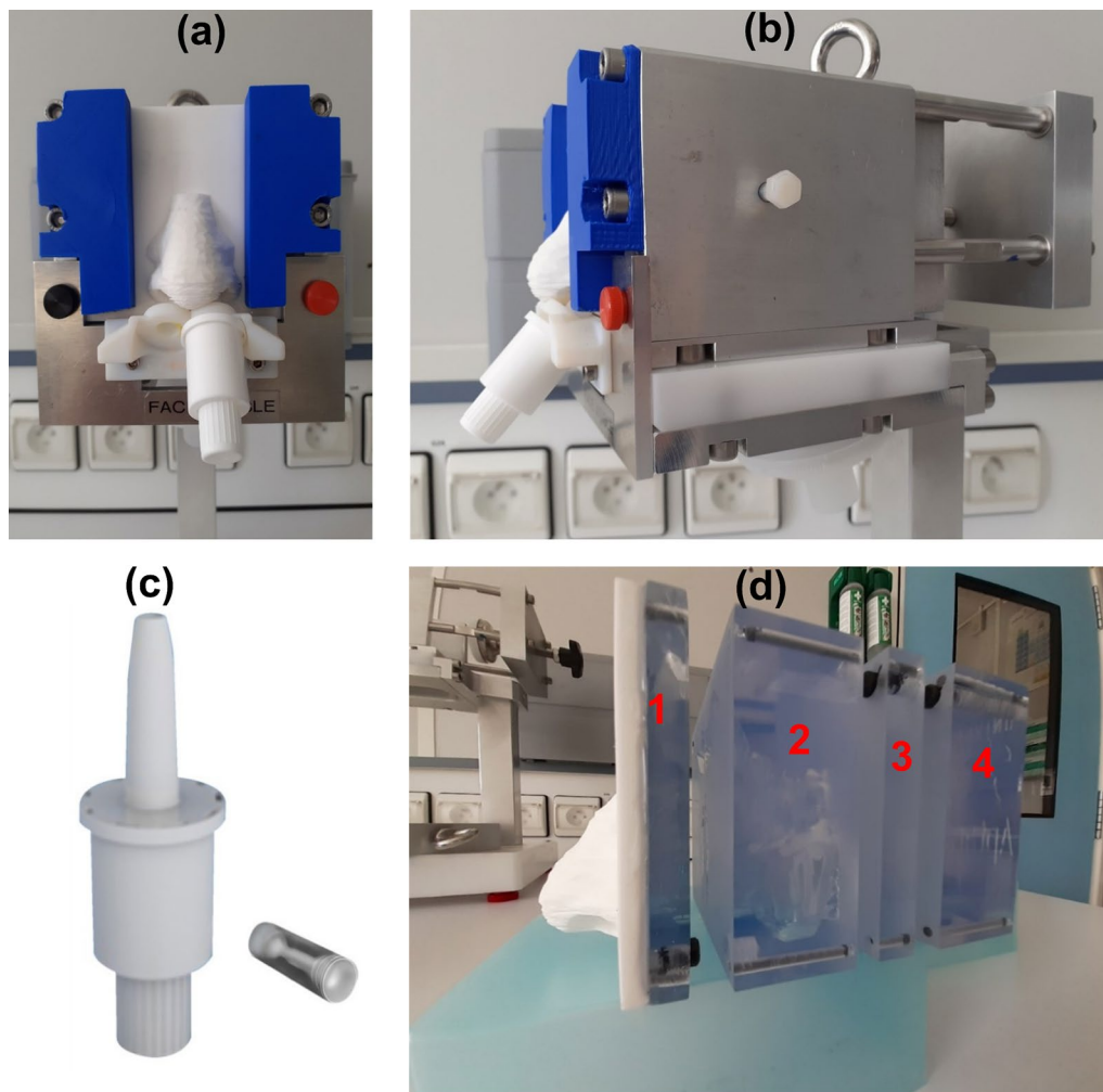
Fig. 2 Nasal cast and spraying device (picture courtesy of Aptar pharma). a, b Pictures of the experimental set-up of artesunate powder deposition study. c Picture of the spraying device (UDSp). d Side picture of the nasal cast showing the nasal cavity divided in 4 blocks (in red): block 1 = nose, nasal valve, and frontal sinuses; block 2 = maxillary sinuses, frontal sinuses, nasal floor, turbinates, and ethmoids; block 3 = maxillary sinuses, sphenoids, nasal floor, ethmoids and turbinates; block 4: Sphenoids and nasopharynx
