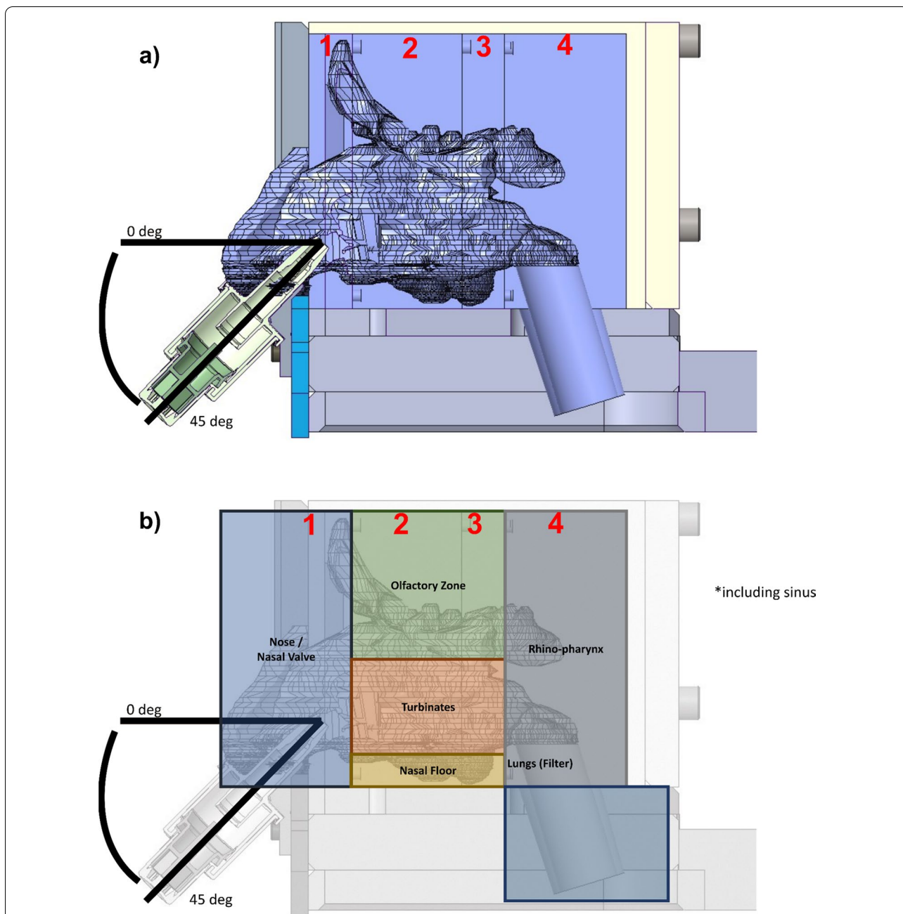
Fig. 3 3D representation of the nasal cast and spray device with the nasal delivery place (picture courtesy of Aptar pharma). a 3D representation of the experimental set-up of artesunate drug deposition study. b 3D representation of the experimental set-up of artesunate drug deposition study with the blocks of the nasal cast and corresponding nasal regions. block 1 = nose, nasal valve, and frontal sinuses; block 2 = maxillary sinuses, frontal sinuses, nasal floor, turbinates, and ethmoid; block 3 = maxillary sinuses, sphenoids, nasal floor, ethmoid and turbinates; block 4: Sphenoids and nasopharynx
