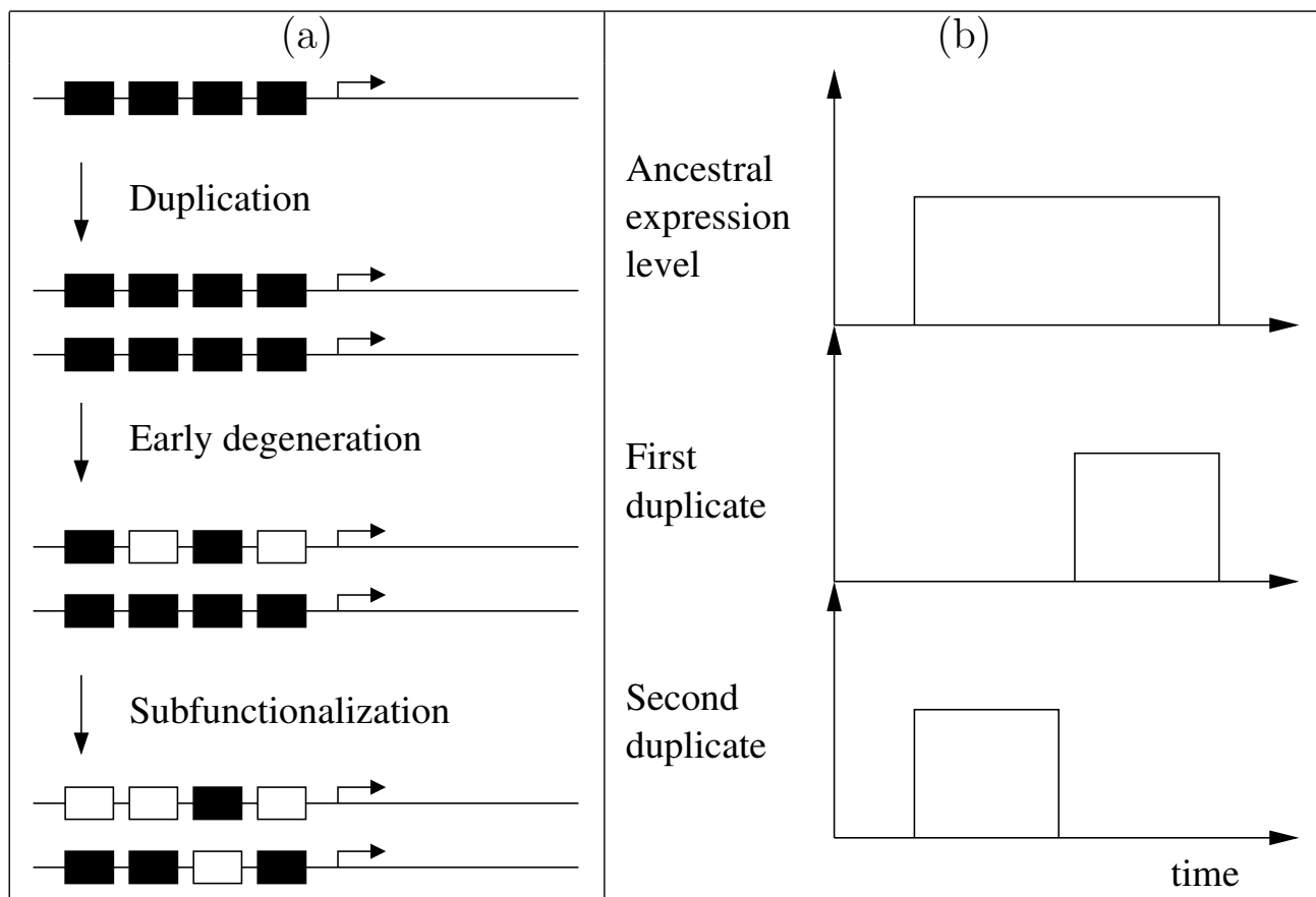
Figure 1 The duplication-degeneration-complementation (DDC) model. (a) A gene with four regulatory elements (black boxes), each controlling independent functions such as expression domains, is duplicated. Random null mutations in the regulatory elements (open boxes) through degeneration lead to subfunctionalization, where the regulatory elements complement each other to achieve the full ancestral repertoire. (b) Temporal subfunctionalization, illustrated here by the temporal expression patterns of a hypothetical ancestor and two evolved duplicates. The expression level of the duplicates has evolved such that the ancestral expression pattern is maintained in complementary temporal domains via the combined expression of the two duplicates.
