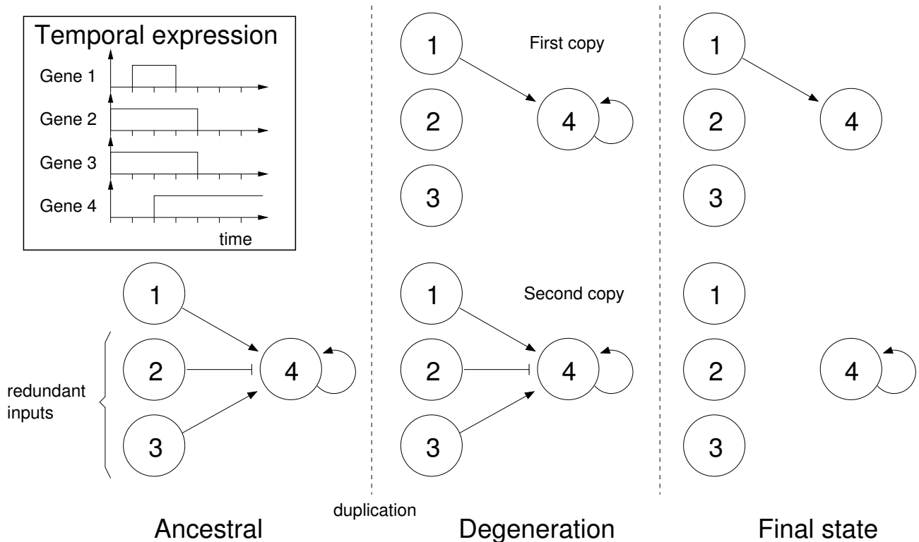
Figure 4 An example of the dominance effect following duplication. The inset (top left) gives an example time course for the protein products of the four genes. Regulation of gene 4 in the ancestral network includes two redundant interactions from genes 2 and 3, which cannot be removed in succession without perturbing the dynamics (since genes 2 and 3 have identical dynamics, their contributions cancel out). However, following duplication, these interactions can be lost successively (albeit in order, with the input from gene 3 degenerating first), since any dynamic perturbations will be masked by the intact second copy. Since the first copy now produces the correct dynamics, the degeneration process can be repeated in the second copy. Further degeneration might lead to a final state of complementation between the two copies.
