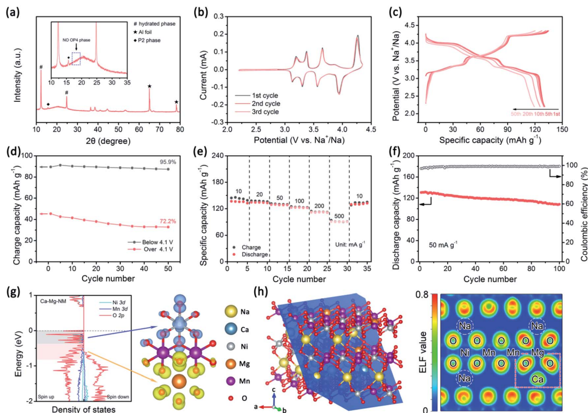
Fig. 6 The properties of the co-doped sample. (a) The XRD pattern at 4.35 V (the inset shows an enlarged view in the range of 10–35°), (b) CV curves, (c) the charge–discharge profiles at 50 \text{ mA g}^{-1} , (d) corresponding charge capacity above and below 4.1 V at 50 \text{ mA g}^{-1} , (e) the rate performance, and (f) the cycling performance at 50 \text{ mA g}^{-1} of \text{Ca}_{0.025} -NMM. (g) The density of states of Ca–Mg–NM at a Na content of 7/27 and the corresponding spatial charge density at -0.37 < E - E_F < 0.00 \text{ eV} and at -0.82 < E - E_F < -0.37 \text{ eV} . (h) The ELF map of Ca–Mg–NM along the blue lattice plane shown in the left panel.
