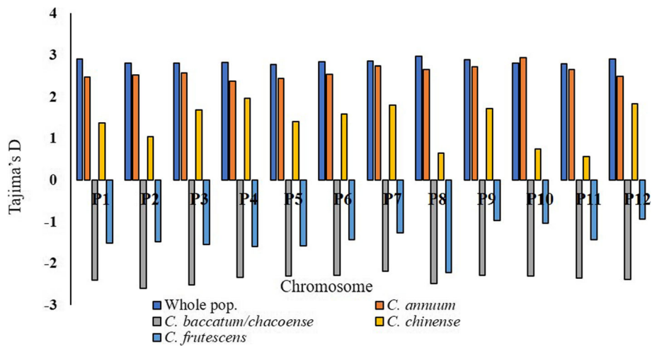
Fig. 3 Tajima's D statistics for each chromosome for the whole Capsicum population and representative species
