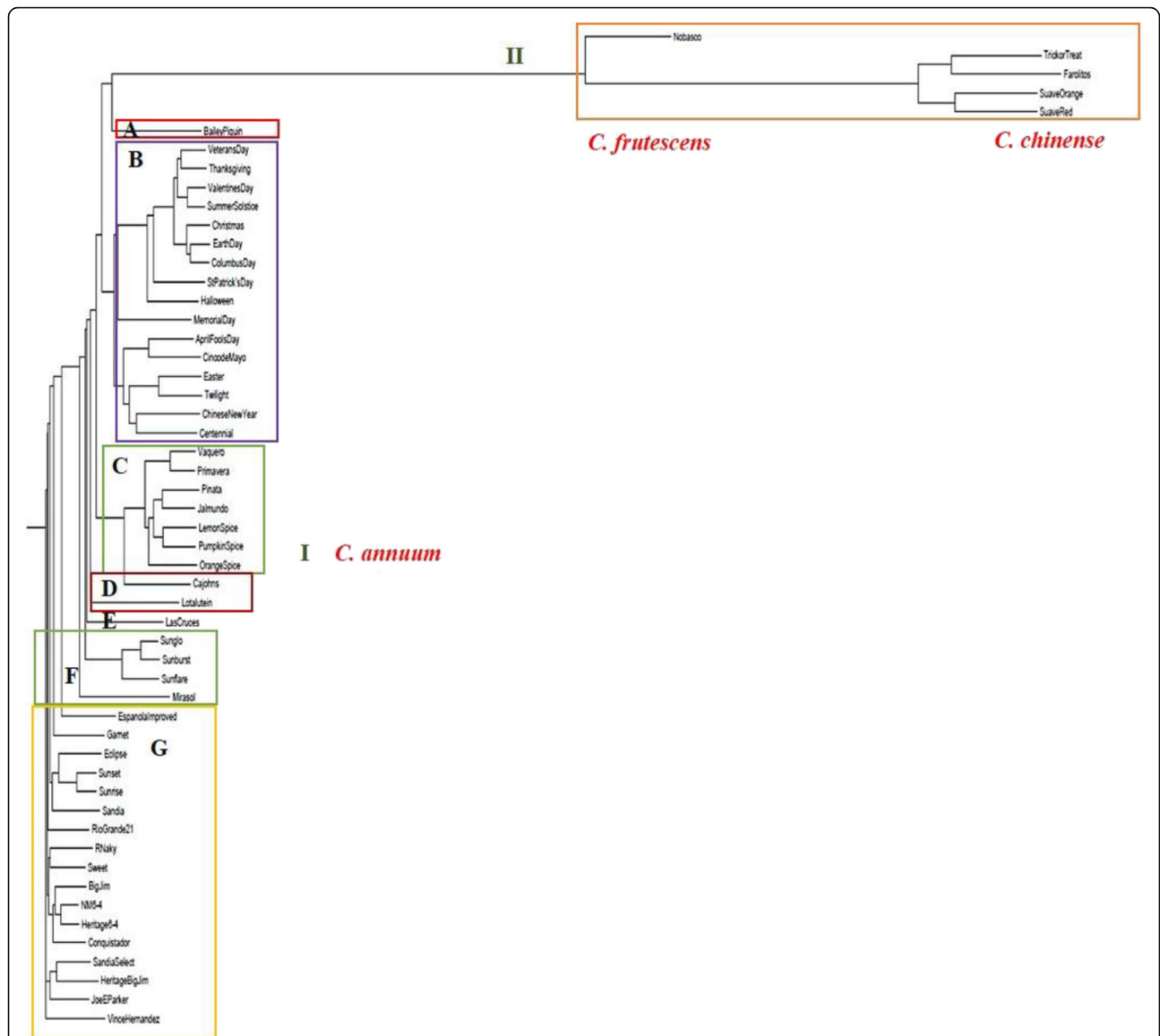
Fig. 2 Neighbor joining (NJ) phylogenetic tree for the NMSU (NuMex) Chile pepper cultivars based on genome wide SNP markers. Cultivars were divided into two major clusters (I and II) according to species. The C. annuum (Cluster I) was separated into seven subgroups (a-g) based on pod (fruit) types: a chile piquin; b ornamental chile peppers; c jalapeno; d serrano; e cayenne; f de arbol; and g New Mexican (includes the paprika type). C. frutescens and C. chinense formed Cluster II that comprised of the tabasco and the habanero types, respectively. Note that the official names for the NMSU Chile pepper cultivars include the designation 'NuMex' before the actual name, e.g. 'Numex Nobasco'. For convenience, the name was omitted in the NJ tree presented herein
