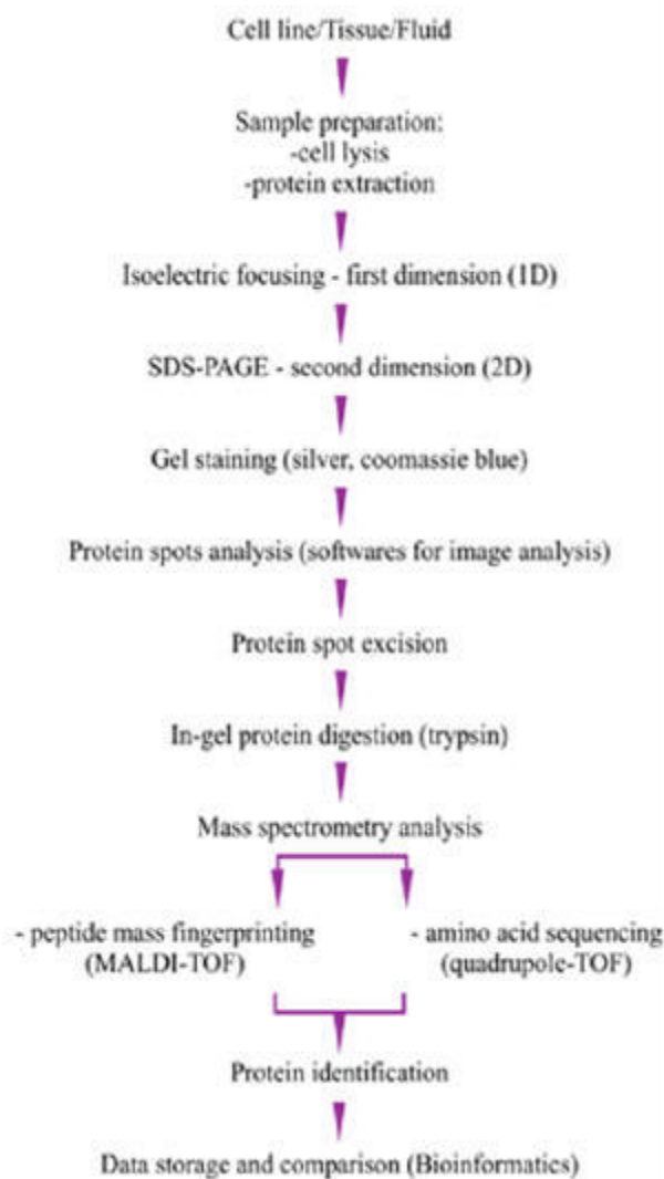
Figure 3. Practical approach to proteome research.
