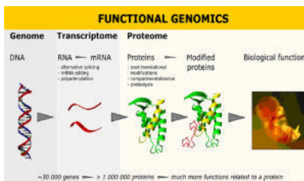
Figure 1. A single gene can give rise to multiple gene products. RNA can be alternatively spliced or edited to form mature mRNA. Besides, proteins are regulated by additional mechanisms such as posttranslational modifications, compartmentalization and proteolysis. Finally, biological function is determined by the complexity of these processes.
