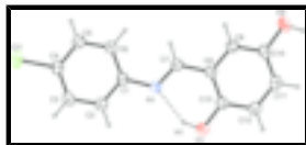
Fig. 1. The molecular structure of the title molecule, with the atom-numbering scheme. Displacement ellipsoids are drawn at the 30% probability level. Hydrogen bonds are shown as dashed lines.
