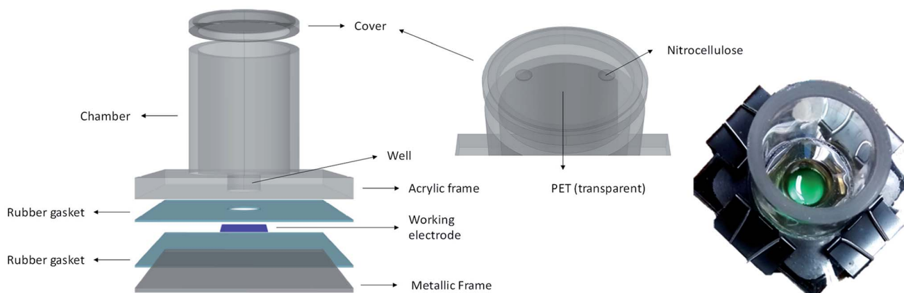
Fig. 2 Schematics and photography of device holding the working electrode.
