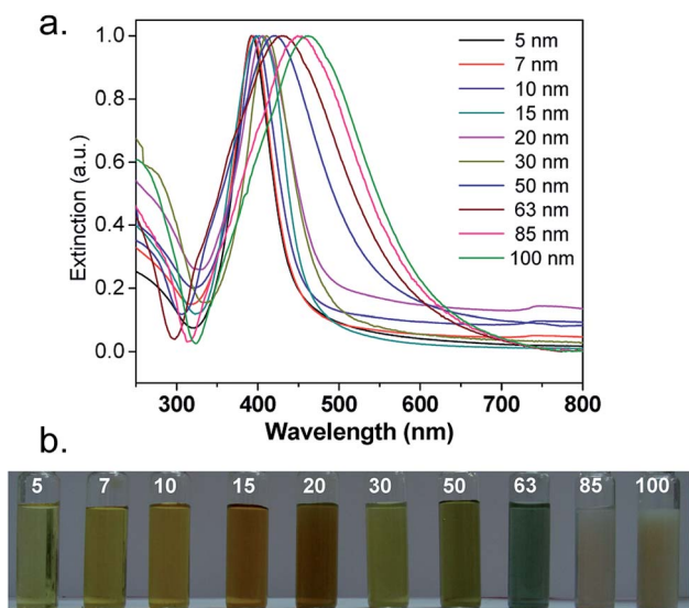
Fig. 4 (a) UV-Vis extinction spectra and (b) the distinctive color of different-sized silver nanoparticles 34b (adapted with permission from Royal Society of Chemistry, 2013).
