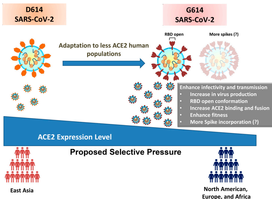
Figure 2. Genetic variability in ACE2 expression as potential driving force for presence of D614G mutation in SARS-CoV-2 S glycoprotein.
