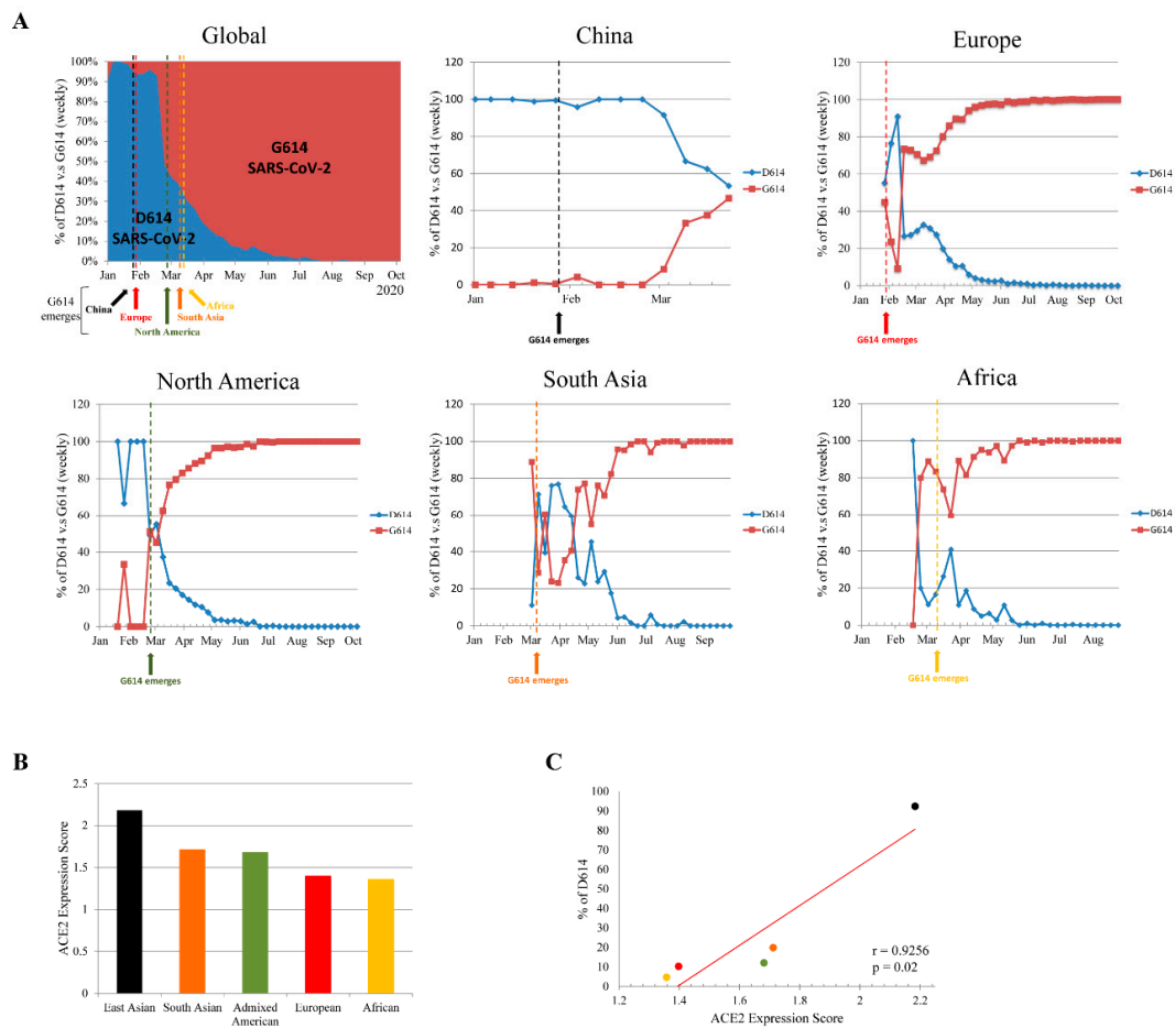
Figure 1. Transition of severe acute respiratory syndrome coronavirus 2 (SARS-CoV-2) spike (S) glycoprotein D614 to G614 variant in different geographic regions. (A) Weekly ratio of D614 and G614 variants globally, and in China, Europe, North America, South Asia, and Africa. Data analyzed from COVID-19 Viral Genome Analysis Pipeline ( https://cov.lanl.gov/ ). (B) Angiotensin 1-converting enzyme 2 (ACE2) expression level in different geographical regions. ACE2 expression score analyzed by 21 ACE2 genetic polymorphisms that significantly affect its expression level according to the current study [18]. (C) Pearson’s correlation coefficient ( r ) and p value between ACE2 expression score and prevalence of D614 variants in different geographical regions.
