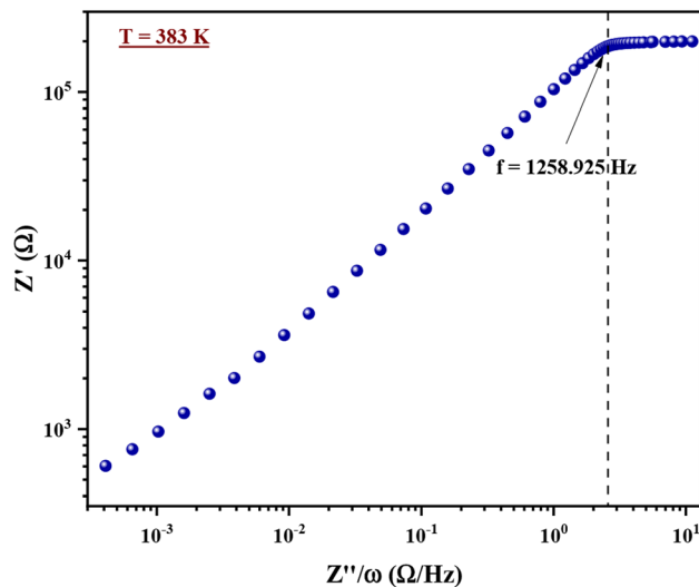
Fig. 7 The relative representation of Z' vs. Z''/\omega at 383 K.
