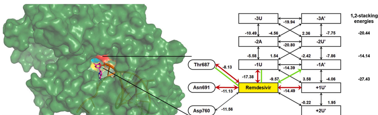
Fig. 2. Interactions established by remdesivir on RdRp based on the remdesivir crystal structure. RdRp is shown as a surface view and colored in green. Remdesivir is shown as a stick model and colored magenta. RNA is shown as a cartoon and colored orange. Thr687 (yellow), Asn691 (cyan), and Asp760 (red) are the amino acids interacting with remdesivir. For clear visibility, 20 % transparency is allowed in the surface view and Lys551 is deleted. Inset figure (right): A diagram of interaction energies between remdesivir, nearby residues, and bases. The square frames represent RNA bases, and the rounded frames signify RdRp residues. The value beside each arrow represents an interaction energy value, with the unit of kcal/mol. The red lines specifically indicate stabilization by hydrogen bonding. The green lines indicate stabilization by \pi - \pi stacking interaction between -1U and -1A' and stabilization by OH/ \pi interaction with Thr687. (For details on the inset figure: see reference [51]) (For interpretation of the references to colour in this figure legend, the reader is referred to the web version of this article).
