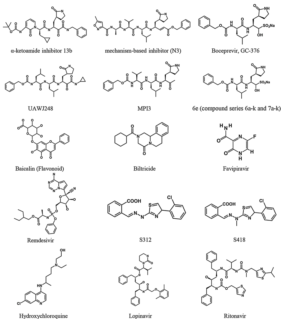
Fig. 1. Chemical structures of small-molecules that have shown significant antiviral activity against SARS-CoV2.
