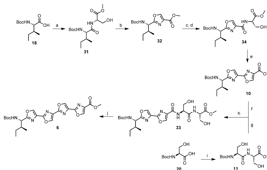
Scheme 7. Reagents and conditions: a) Ser-OMe-HCl ( 19 ), HOBT, EDCI, NiPr 2 Et, CH 2 Cl 2 , RT, 20 h, 91%; b) Deoxo-Fluor, CH 2 Cl 2 , -20°C, 30 min, then BrCCl 3 , DBU, 2-3°C, 8 h, 81%; c) LiOH·H 2 O, THF/MeOH/H 2 O (5:5:1), 0°C→RT, 18 h; d) Ser-OMe-HCl ( 19 ), HOBT, EDCI, NiPr 2 Et, CH 2 Cl 2 , RT, 20 h, 82% (2 steps); e) Deoxo-Fluor, CH 2 Cl 2 , -20°C, 30 min, then BrCCl 3 , DBU, 2-3°C, 7 h, 78%; f) LiOH·H 2 O, THF/MeOH/H 2 O (10:6:1), 0°C→RT, 2 h; g) HCl, 1,4-dioxane, 0°C→RT, 3.5 h; h) HOBT, EDCI, NiPr 2 Et, CH 2 Cl 2 , RT, 20 h, 61% (3 steps); i) Ser-OMe-HCl ( 19 ), HOBT, EDCI, NiPr 2 Et, CH 2 Cl 2 , RT, 20 h, 88%; j) Deoxo-Fluor, CH 2 Cl 2 , -20°C, 45 min, then BrCCl 3 , DBU, 0°C, 24 h, 77%.
