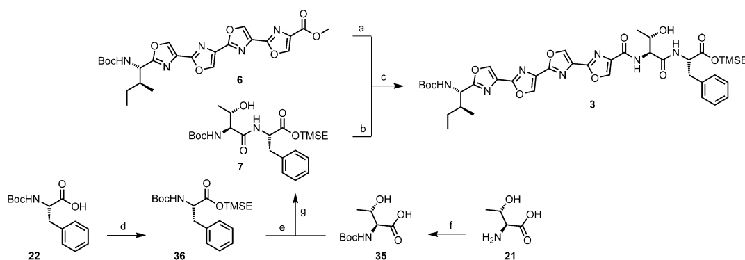
Scheme 8. Reagents and conditions: a) LiOH·H 2 O, CHCl 3 /MeOH/H 2 O (9:3:1), 68°C, 48 h; b) HCl, 1,4-dioxane, 0°C→RT, 4 h; c) HATU, NiPr 2 Et, CH 2 Cl 2 , DMF, 0°C→RT, 18 h, 77% (3 steps); d) (CH 3 ) 3 SiCH 2 CH 2 OH, EDCI, DMAP, CH 2 Cl 2 , 0°C→RT, 18 h, 74%; e) HCl, 1,4-dioxane, 0°C→RT, 30 min; f) NaHCO 3 , Boc 2 O, H 2 O, MeOH, RT, 15 h; g) HATU, NiPr 2 Et, CH 2 Cl 2 , 0°C→RT, 15 h, 81% (3 steps).
