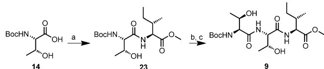
Scheme 2. Reagents and conditions: a) Ile-OMe-HCl ( 17 ), HOBT, EDCI, NiPr 2 Et, CH 2 Cl 2 , RT, 19 h, 99%; b) HCl, 1,4-dioxane, RT, 23 h; c) Boc-Thr-OH ( 14 ), HOBT, EDCI, NiPr 2 Et, CH 2 Cl 2 , RT, 18 h, 79% (2 steps).
