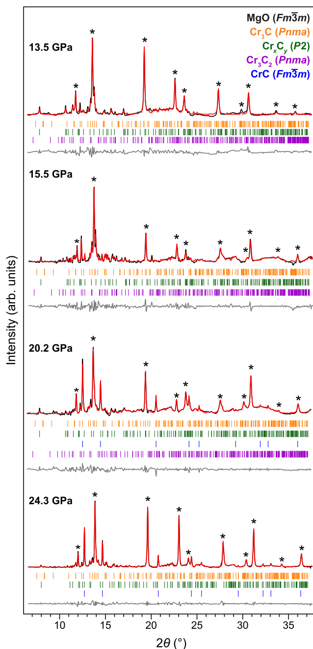
Figure 4. X-ray diffraction measured after thermal quenching at each heating site. Background subtracted experimental data are plotted in black. Rietveld methods are used to fit the multiple phases present and to extract unit cell parameters, with the modeled intensities plotted in red. Residual intensity is plotted in gray. Ticks are plotted beneath each trace to indicate the peak positions of the refined phases and are color-coded to each phase as denoted in the inset legend. Asterisks mark reflections from \text{MgO} ( Fm \bar{3}m ).
