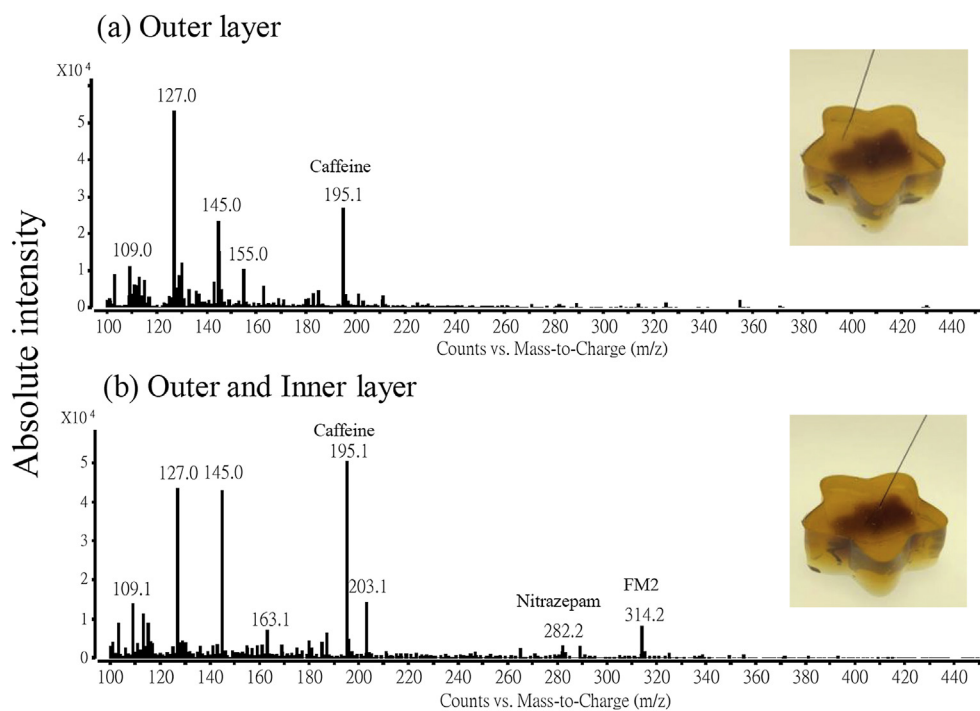
Fig. 4 – TD-ESI mass spectra for a jelly candy. To collect the sample, an acupuncture needle was (a) inserted into the outer star-shaped layer and (b) pierced through the outer layer to insert into the inner gummy bear.
