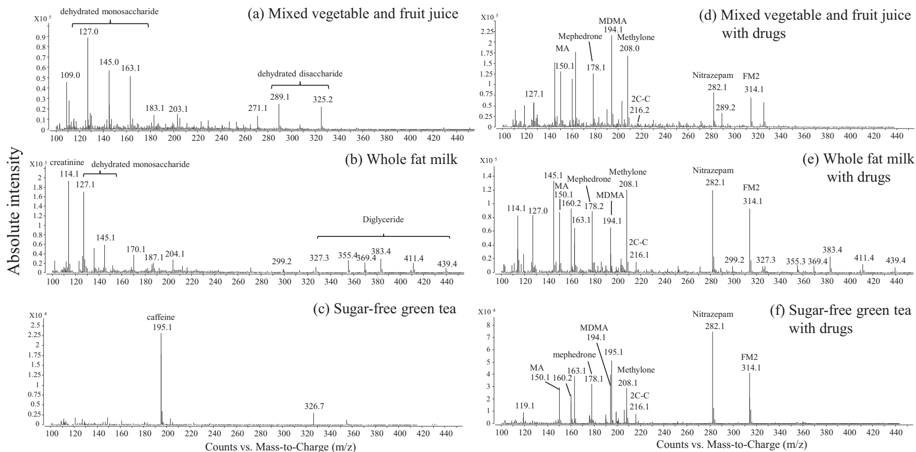
Fig. 1 – TD-ESI mass spectra for (a, d) fruit and vegetable juice, (b, e) whole fat milk, and (c, f) sugar free green tea laced (a–c) without or (d–f) with illicit drugs (MA, mephedrone, MDMA, methylone, 2C-C, nitrazepam, and FM2; each at 100 ppm), respectively.
