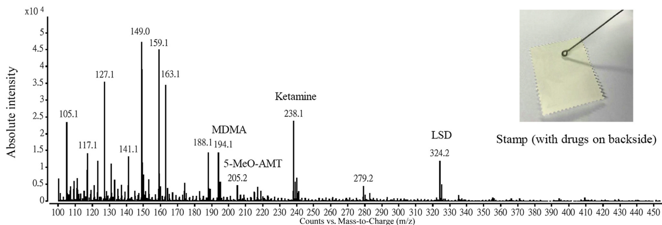
Fig. 3 – TD-ESI mass spectrum for a stamp with ketamine, MDMA, 5-MeO-AMT, and LSD applied on the backside of stamp surface (each 5.2 ng/mm 2 ).
