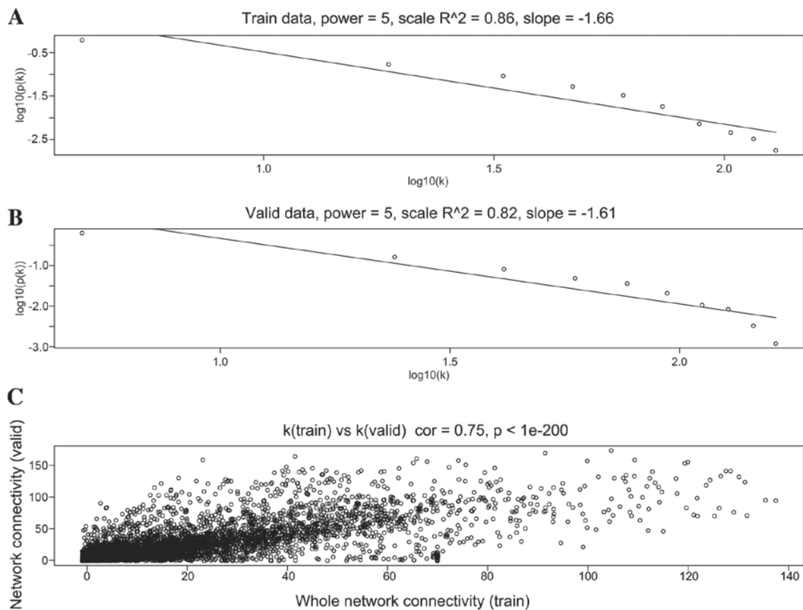
Figure 2. Distribution of genes in terms of degree (soft threshold, 5). (A) Training set; (B) Validation set; X-axis indicates degree k ; Y-axis indicates percentage of genes with degree k . (C) Correlation between the training dataset and validation dataset co-expression networks. The x-axis indicates degree k in the training dataset; y-axis indicates degree k in the validation dataset.
