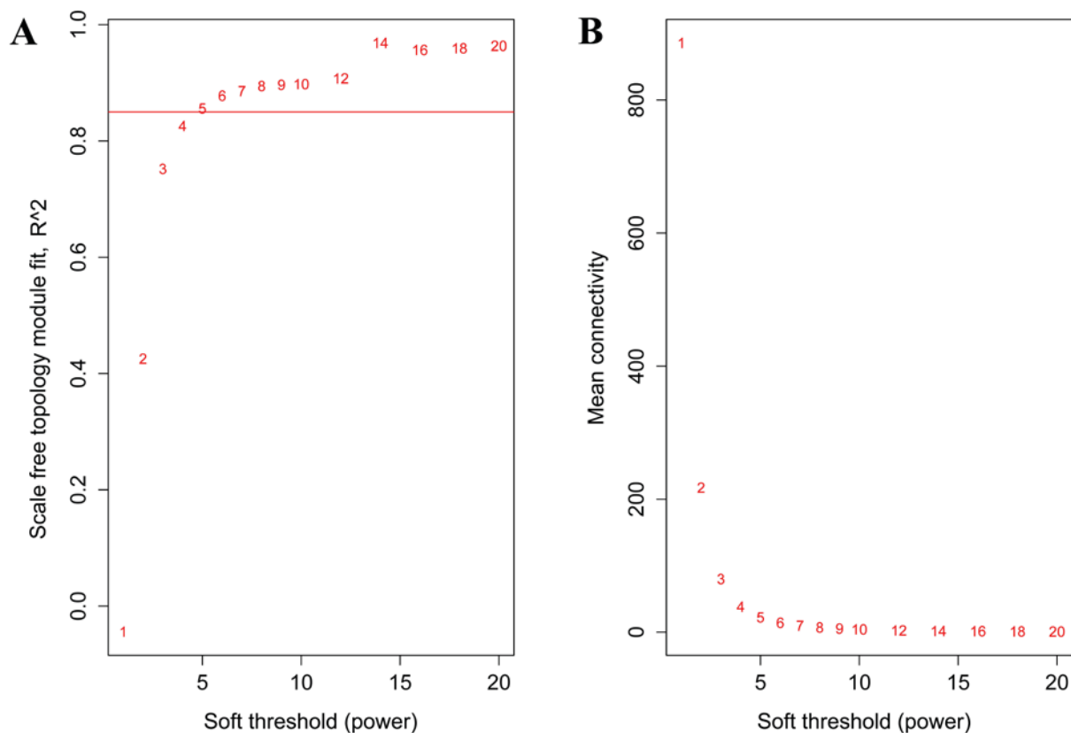
Figure 1. (A) Scale-free fit R^2 vs. various soft thresholds. The red line indicates an R^2 of 0.85. (B) Mean Connectivity vs. different soft threshold \beta .
