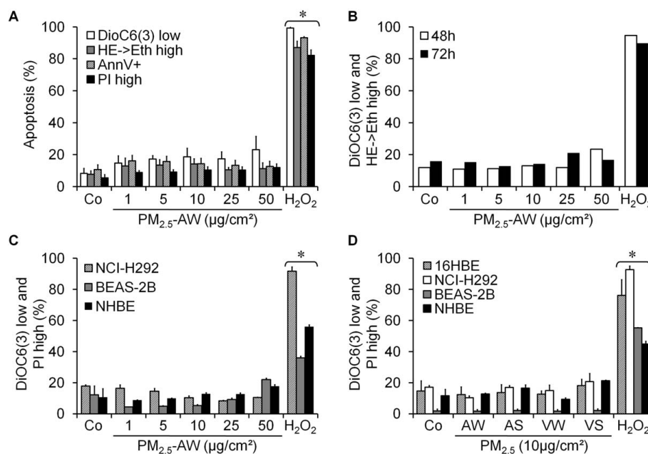
Figure 1 Effect of PM 2.5 -AW exposure on human bronchial epithelial cells. (A) Dose response of DiOC6(3) (to measure the mitochondrial ΔΨ m drop), hydroethidine (HE, ROS-sensitive dye), Annexin V-FITC (for phosphatidylserine exposure) and the propidium iodide (PI, as a plasma membrane permeabilization marker) staining after 24 hours exposure of 16HBE bronchial epithelial cells to PM 2.5 -AW (1-50 μg/cm 2 ) or H 2 O 2 (500 μM). (B) Kinetic study of PM 2.5 -AW effect on apoptosis. 16HBE cells were exposed to PM 2.5 -AW (1 to 50 μg/cm 2 ) or H 2 O 2 (500 μM) before flow cytometric analysis of cells presenting simultaneously a mitochondrial depolarization (DiOC6(3) low) and a superoxide anion generation (HE → Eth high). Results are representative of three independent experiments. (C) Subconfluent bronchial epithelial cell lines NCI-H292, BEAS-2B and primary bronchial epithelial cells (NHBE) were exposed 24 h to 1-50 μg/cm 2 PM 2.5 -AW, and H 2 O 2 (1 mM) before flow cytometric analysis of cells presenting simultaneously a DiOC6(3) low and PI high staining. (D) Human bronchial epithelial cells 16HBE, NCI-H292, BEAS-2B and primary bronchial epithelial cells (NHBE) were exposed 24 hours to 10 μg/cm 2 of different batches of PM 2.5 (Auteuil-Winter (AW), Auteuil-Summer (AS), Vitry-Winter (VW) or Vitry-Summer (VS) corresponding to two locations of Paris: (i) a school playground at Vitry-sur-Seine in a suburb of Paris and (ii) Porte d'Auteuil adjacent to a major highway). Then, cells were analyzed as previously described. Data are represented as mean ± SD (* treated vs. control, p < 0.05, n = 3).
