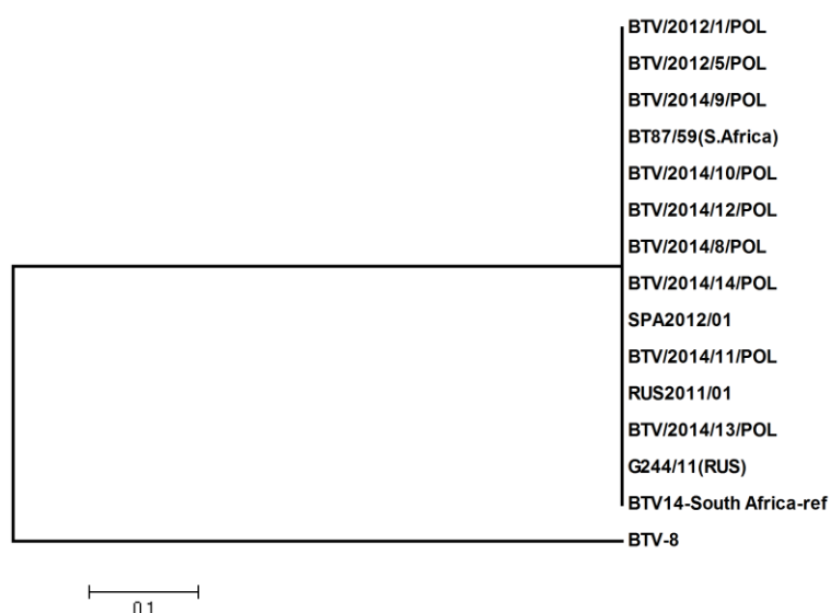
Fig. 1. The phylogenetic tree comparing the Polish BTV-14 isolates with the reference BTV-14 strains. The phylogenetic analysis was conducted with the NJ method. Bootstrap values were obtained for 1,000 replicates. The BTV-8 strain was used as the outgroup
