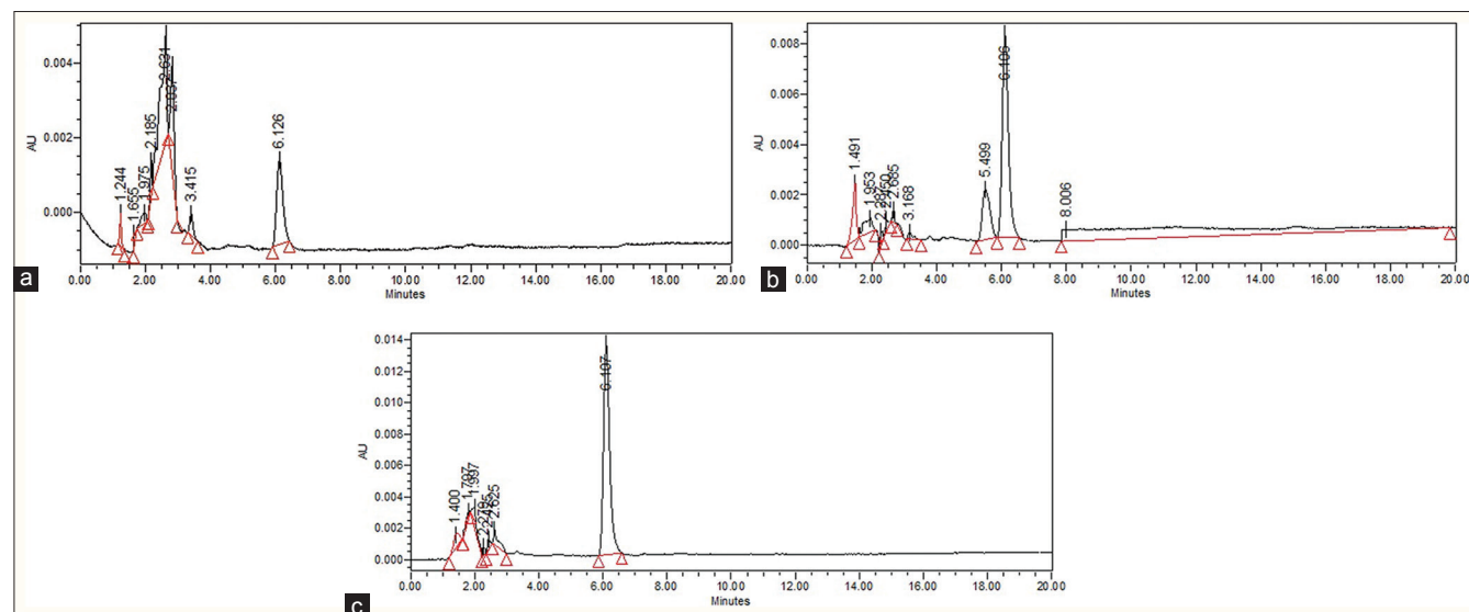
Figure 3: RP-HPLC chromatogram for stress-induced Withanolide A standard (a) alkali treatment (b) acid treatment (c) peroxide treatment
