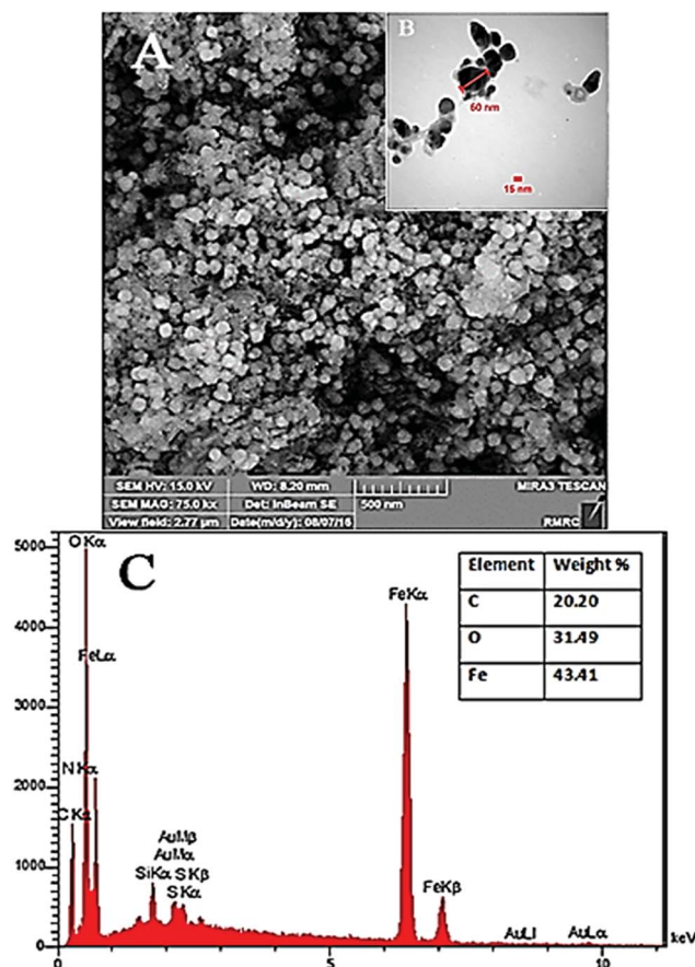
Fig. 4 (A) SEM image, (B) TEM image and (C) EDS results showing the presence of zero valent iron nanoparticles and the bio-organic components of M. communis leaf extract.
