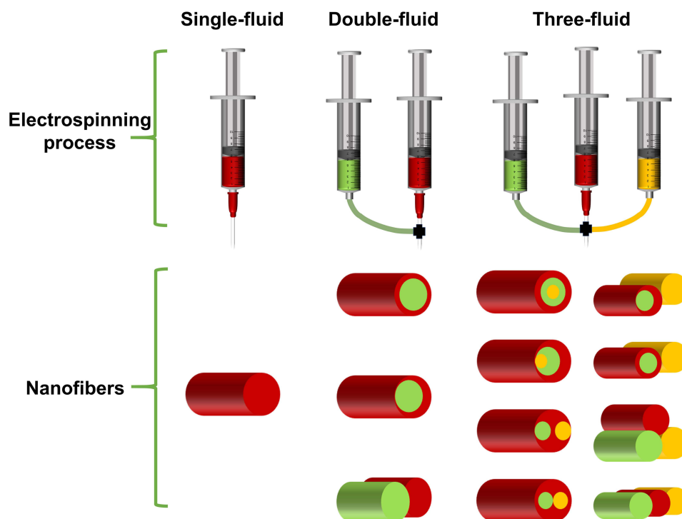
Figure 4 Schematic diagram of the electrospinning process classification and their respective fiber structure.
