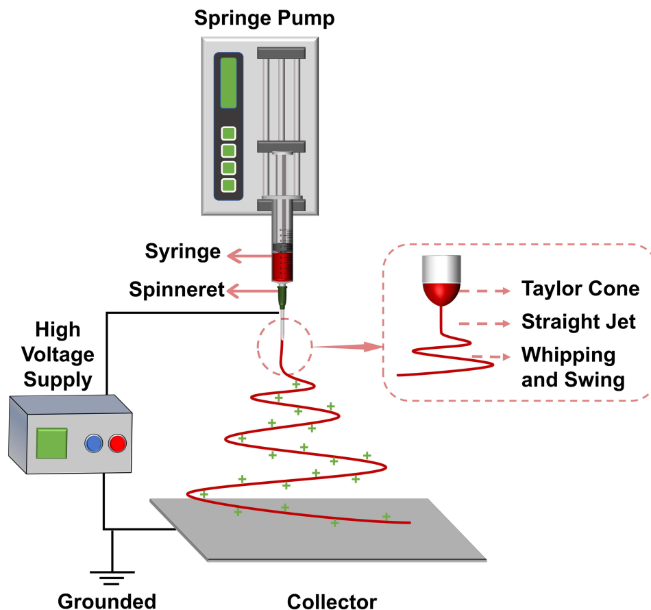
Figure 3 Electrospinning device and the schematic diagram of the electrospinning process.
