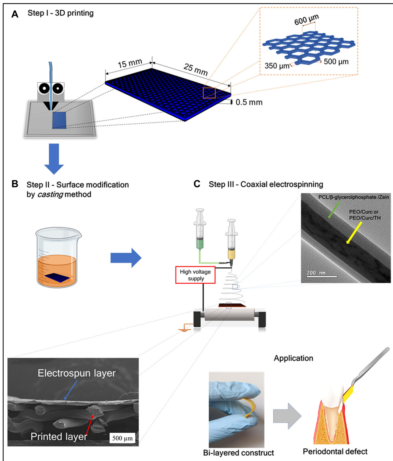
Figure 14 Design of electrospinning and 3D printing bilayer structure. (A) The first step of PLA 3D printing honeycomb platform. (B) In the second step, the honeycomb walls were modified with a zein-based membrane using the casting method. (C) The third step deposits a coaxial electrospun fiber layer on one surface of the 3D printed modified structure. Reproduced with permission from dos Santos DM, de Annunzio SR, Carmello JC, et al. Combining coaxial electrospinning and 3D printing: design of biodegradable bilayered membranes with dual drug delivery capability for periodontitis treatment. ACS Appl Bio Mater. 2022;5(1):146–159. Copyright © 2022 American Chemical Society. 162
