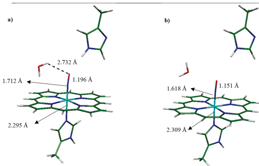
Fig. 1 Optimized structure and model system for (a) [\text{MI-Fe}^{\text{II}}\text{P-NO}\cdots\text{MI}] and (b) [\text{MI-Fe}^{\text{III}}\text{P-NO}\cdots\text{MI}]^+ determined at the OPBE/DZVP-GGA/GEN-A2* level of theory.
