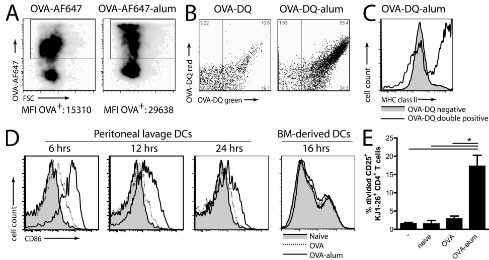
Figure 4. Alum adjuvant stimulates DC function in vivo. (A) Mice were injected i.p. with OVA-Alexa Fluor 647 (OVA-AF647) or OVA-AF647-alum. 24 h after injection, the peritoneal lavage was taken and the uptake of OVA-AF647 was assessed in F4/80^{-}MHCII^{+}CD11c^{+} DCs. (B) Mice were injected with OVA-DQ or OVA-DQ-alum i.p., and 24 h later, the mDCs ( F4/80^{-}MHCII^{+}CD11c^{+} ) in the peritoneal lavage were analyzed for the uptake and processing of DQ by flow cytometry. OVA-DQ fluoresces green when processed in acidified lysosomes. Red fluorescence is caused by accumulation of OVA-DQ in endosomal processing compartments in the cell. (C) The CD11c^{+} cells were also analyzed for the expression of MHCII in the DQ-negative or -double-positive gate. Gray-filled histograms represent OVA-DQ-negative, and black line histograms represent OVA-DQ-double-positive CD11c^{+} cells. (D) Maturation of mDCs in the peritoneal lavage was assayed 6, 12, and 24 h after injection of OVA or OVA-alum by flow cytometry. BM-derived DCs (BM-DCs) were pulsed for 16 h with OVA or OVA-alum. Gray filled histograms represent naive mice or unpulsed BM-DCs, black dotted line histograms represent OVA-injected mice or OVA-pulsed BM-DCs, and black solid line histograms represent OVA-alum-injected mice or OVA-alum-pulsed BM-DCs. (E) Mice were injected with OVA or OVA-alum, and 6 h later, the F4/80^{-}MHCII^{+}CD11c^{+} DCs were sorted from the peritoneal lavage and placed in co-culture with CFSE-labeled DO11.10 Tg CD4^{+} T cells. After 4 d, cells were analyzed for proliferation and gated for CD4^{+} , KJ1-26^{+} , and CD25^{+} .
