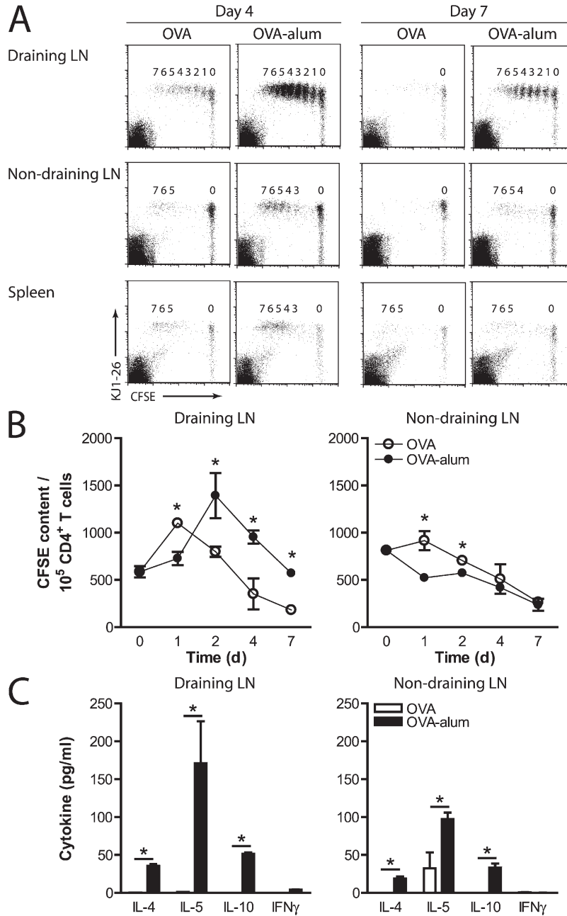
Figure 2. Addition of alum adjuvant to OVA leads to a stronger, more persistent and recirculating Th2 immune response. Mice were injected with CFSE-labeled D011.10 OVA-TCR Tg cells 1 d before the i.p. injection of OVA or OVA-alum. (A) 4 and 7 d after the injection the DLN (MLN), nondraining LN (CLN), and the spleen were analyzed for T cell proliferation with flow cytometry ( n = 4 mice; experiment performed three times). (B) CFSE content was calculated as described in Materials and methods, and is shown for DLN (MLN) and nondraining LN (ALN). Open symbols represent the OVA-injected mice, and the filled symbols the OVA-alum injected mice. (C) 7 d after the i.p. injection, LN cells (DLN: MLN, nondraining LN: ALN) were taken and restimulated in vitro for 4 d with OVA. Cytokines were measured in the supernatants by ELISA. Open bars represent OVA-injected mice, and closed bars represent the OVA-alum-injected mice. Data are shown as the mean \pm the SEM, *, P < 0.05 . n = 4-6 mice per group.
