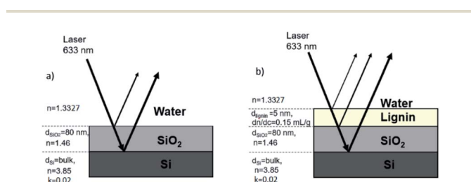
Fig. 2 Overview of parameters in the multilayer optical model describing the reflection interface.
