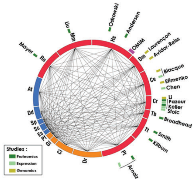
Figure 1. Orthology calculations and links to ciliary studies underlying Cildb. The 18 species analyzed are represented as circle arcs proportional to the size of the proteome, in red when ciliary studies exist (delineated as ticks outside the circle), in orange when centriole/cilia exist, but without high throughput studies, and in blue when no cilia or centriole exists (At: Arabidopsis thaliana ; Ce: Caenorhabditis elegans ; Ci: Ciona intestinalis ; Cr: Chlamydomonas reinhardtii ; Dd: Dictyostelium discoideum ; Dm: Drosophila melanogaster ; Dr: Danio rerio ; Ec: Escherichia coli ; Gl: Giardia lamblia ; Hs: Homo sapiens ; Mm: Mus musculus ; Pf: Plasmodium falciparum ; Pt: Paramecium tetraurelia ; Rn: Rattus norvegicus ; Sc: Saccharomyces cerevisiae ; Sp: Schizosaccharomyces pombe ; Tb: Trypanosoma brucei ; Tt: Tetrahymena thermophila ). The colors of the ticks for the studies are explained in the inset to distinguish proteomic, transcriptomic and comparative genomic studies. Andersen (35); Arnaiz [this article for proteomics, or Arnaiz et al. (in preparation) for transcriptome analysis]; Avidor-Reiss (36); Blacque (37); Broadhead (38); Chen (39); Efimenko (40); Keller (41); Kilburn (42); Laurencon (43); Li (16); Liu (44); Mayer (45); Ostrowski (19); Pazour (26); Smith (18); Stolc (46). For each species, the whole proteome was compared by BLASTp to itself and to all the other ones, in order to apply our three orthology filters (Inparanoid, Inparanoid + filtered best hits, BLASTp cutoff), as described in experimental procedures. The high throughput ciliary studies were then remapped to the proteins, so that links between orthology and ciliary properties are created. The genome versions and the origin of the ciliary study data in Cildb are reported in Supplementary Table S1. The human genome is also linked to the OMIM database in which genetic disorders appear.
