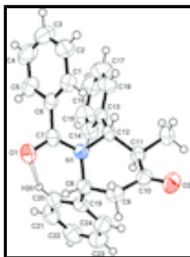
Fig. 1. ORTEP diagram of the title compound with 50% probability displacement ellipsoids. Dotted bond indicates the intramolecular C—H \cdots O hydrogen bond.
