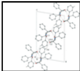
Fig. 2. Crystal packing diagram of the title compound. The dotted lines indicate intermolecular C—H...O hydrogen bonds.
