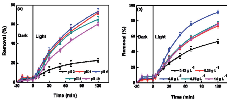
Fig. 4 Experimental parameters investigation for the photocatalytic degradation of crystal violet with BUT-206 : (a) effect of pHs (2–10) on the photocatalytic degradation performance; (b) effect of dose of MOF ( 0.12\text{--}1.0 \text{ g L}^{-1} ) on the photocatalytic degradation performance.
