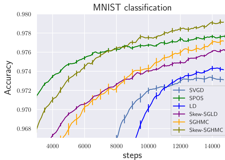
Figure 6. MNIST classification (Averaged over ten trials).
