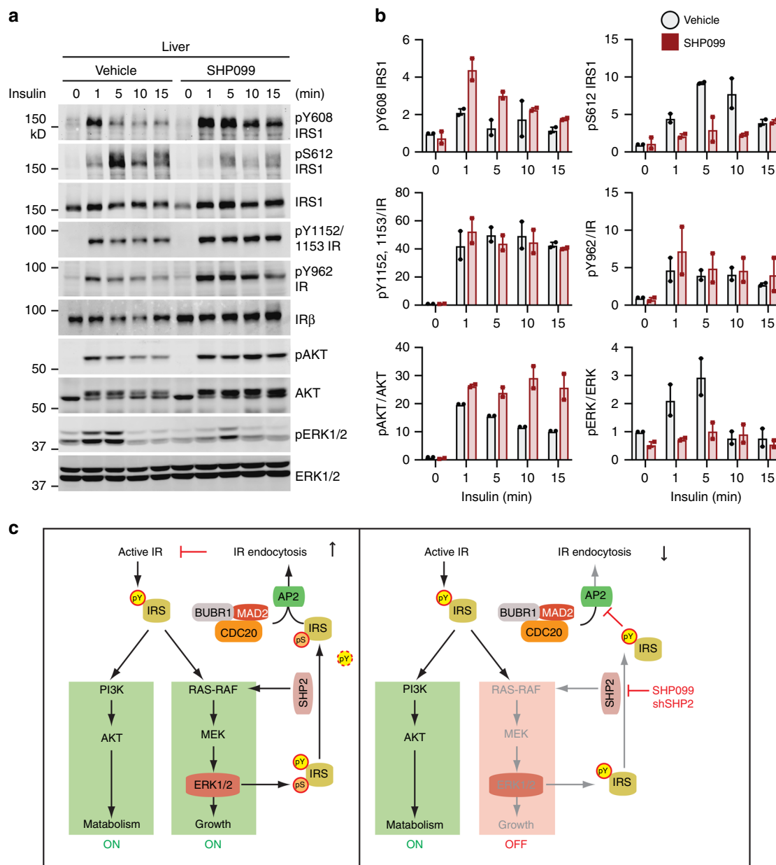
Fig. 8 Mitotic regulators and SHP2 promote feedback inhibition of IR. a Insulin signaling in the liver from mice fed HFD for 5 weeks. The mice were administered vehicle or SHP099 for 5 days, fasted overnight, and administered vehicle or SHP099 once more. At 2 h after the last administration, the mice were injected with or without 1U insulin via inferior vena cava. The livers were collected at the indicated time points. Lysates were prepared from these tissues and subjected to quantitative immunoblotting with the indicated antibodies. b Quantification of the blots in a . Mean \pm range; n = 2 independent experiments. c Targeting feedback regulation of IR endocytosis for diabetes treatment. Left panel depicts the feedback regulation of IR endocytosis by ERK1/2 and SHP2 during unperturbed insulin signaling. Right panel illustrates the mechanism by which SHP2 inhibitor (SHP099) or shRNA blocks growth-promoting IR signaling and IR endocytosis, and prolongs insulin signaling through the PI3K-AKT pathway, which controls metabolism. Source data are provided as a Source Data file
