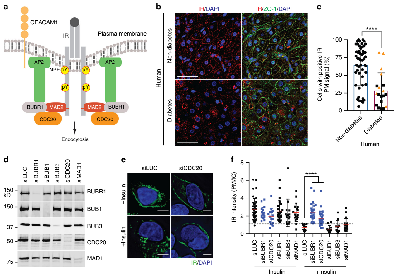
Fig. 1 CDC20 is required for insulin-activated IR endocytosis. a Model of the regulation of IR endocytosis by spindle checkpoint proteins. MIM, MAD2-interacting motif. b Representative images of liver specimens from human non-diabetic and diabetic patients stained with DAPI (blue) and anti-IR (red) and anti-ZO-1 (green) antibodies. Scale bars, 40 \mu m. c Quantification of the percentage of cells with positive IR PM signals in liver specimens in b (non-diabetes, n = 51 ; diabetes, n = 19 ; mean \pm s.d.; **** p < 0.0001 ; Mann-Whitney test, a non-parametric test). The liver specimens from insulin-treated patients were presented as orange triangles. d Western blot analysis of lysates of HepG2 cells stably expressing IR-GFP WT that had been transfected with the indicated siRNAs. e Cells in d were serum starved, treated without or with 100 nM insulin for 5 min, and stained with anti-GFP antibodies. Scale bar, 5 \mu m. f Quantification of the ratios of PM and IC IR-GFP signals of cells in e (siLuc, n = 39 ; siLuc + Ins, n = 14 ; siBUBR1, n = 18 ; siBUBR1 + Ins, n = 29 ; siCDC20, n = 17 ; siCDC20 + Ins, n = 34 ; siBUB1, n = 23 ; siBUB1 + Ins, n = 12 ; siBUB3, n = 15 ; siBUB3 + Ins, n = 10 ; siMAD1, n = 19 ; siMAD1 + Ins, n = 18 ; mean \pm s.d.; **** p < 0.0001 ; two-tailed unpaired t test). Source data are provided as a Source Data file
