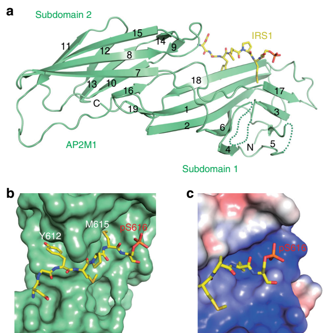
Fig. 6 The crystal structure of AP2M1 bound to pS616-IRS1. a Ribbon diagram of the crystal structure of AP2M1 (residues 160–435) bound to pS-IRS1. pS-IRS1 is shown as sticks. b Surface drawing of AP2M1, with pS-IRS1 shown as sticks. c A close-up view of the surface drawing of AP2M1 colored by its electrostatic potential (blue, positive; red, negative; white, neutral). pS-IRS1 is shown as sticks
