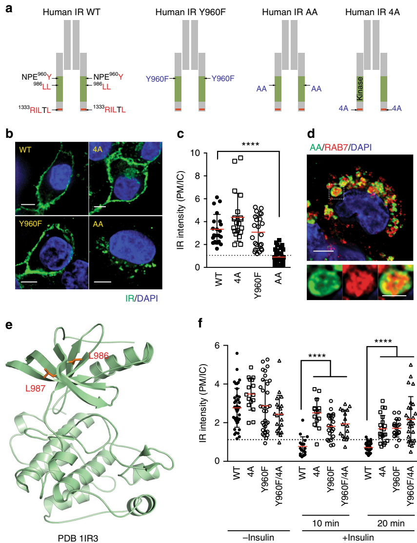
Fig. 3 The NPEY motif and MIM of IR are required for endocytosis. a Schematic illustration of sequence motifs and mutants of IR \beta . b HepG2 cells stably expressing IR-GFP WT, 4A, Y960F, or AA were serum starved and stained with anti-GFP antibodies. Scale bars, 5 \mu m. c Quantification of the ratios of plasma membrane (PM) and intracellular (IC) IR-GFP signals of cells in b (WT, n = 21 ; 4A, n = 20 ; Y960F, n = 23 ; AA, n = 32 ; mean \pm s.d.; **** p < 0.0001 ; two-tailed unpaired t test). d HepG2 cells stably expressing IR-GFP AA were serum starved and stained with anti-GFP and anti-RAB7 antibodies. Scale bar, 5 \mu m. The boxed region was magnified and shown on the right. Scale bar in the boxed region, 2.5 \mu m. e Ribbon diagram of the crystal structure of the IR kinase domain, with L986 and L987 shown as sticks. f HepG2 cells stably expressing IR-GFP WT, 4A, Y960F, or Y960F/4A were serum starved, treated without or with 100 nM insulin for the indicated durations, and stained with anti-GFP antibodies. Quantification of the ratios of PM and IC IR-GFP signals of cells was shown (WT, n = 40 ; WT + Ins, 10 min, n = 17 ; WT + Ins, 20 min, n = 33 ; Y960F, n = 32 ; Y960F + Ins, 10 min, n = 21 ; Y960F + Ins, 20 min, n = 19 ; 4A, n = 16 ; 4A + Ins, 10 min, n = 15 ; 4A + Ins, 20 min, n = 21 ; Y960F + 4A, n = 20 ; Y960F + 4A + Ins, 10 min, n = 16 ; Y960F + 4A + Ins, 20 min, n = 27 ; mean \pm s.d.; **** p < 0.0001 ; two-tailed unpaired t test). Source data are provided as a Source Data file
