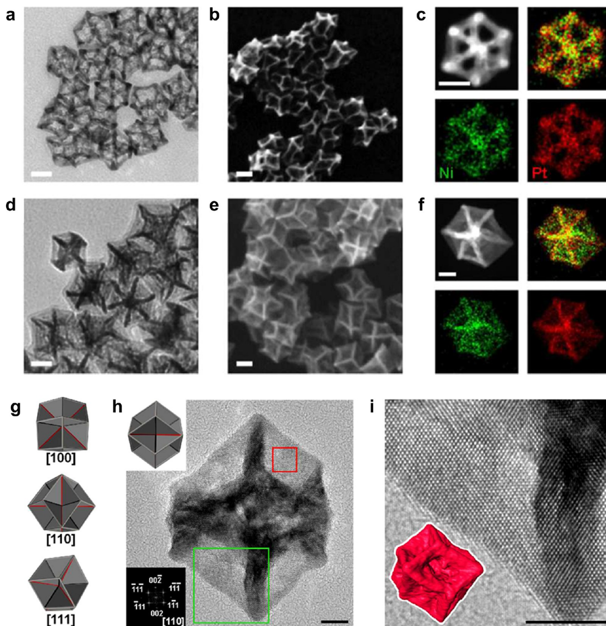
Figure 13. TEM and SEM images of (a, b) a hollow nanoframe and (d, e) a excavated nanoframe (E-NF). STEM-HAADF image and STEM-EDS mapping of (c) a hollow nanoframe and (f) a excavated nanoframe oriented in the \langle 111 \rangle direction. (g) Model of E-NF shown in three orientations. (h) HRTEM image of E-NF oriented in the \langle 110 \rangle direction. The top left inset is the corresponding model of ENF in the identical orientation. The bottom left inset is the FFT of the image in the red box. (i) Magnified HRTEM image of thin sheet in E-NF from green box in (h), with high-tilt angle STEM tomography rendering of E-NF in the inset. Scale bars represent 10 and 5 nm for (a–f) and (h, i), respectively. Reprinted with permission from ref 99, 2017, American Chemical Society.
