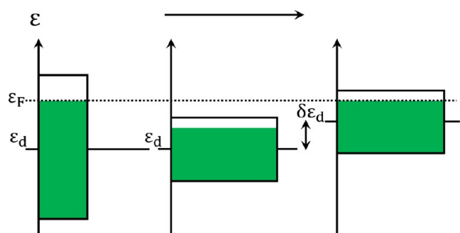
Figure 9. Schematic illustration of the coupling between bandwidth and d-band center for a band with a fixed number of d-electrons. When the bandwidth is decreasing, the only way of maintaining the number of d-electrons is to shift up the center of the band. Reproduced with permission from ref 65, 2007, Elsevier.
