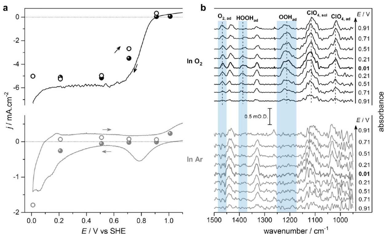
Figure 19. (a) Comparison of voltammetry (lines, scan rate 2 mV s -1 ) and average current densities ( j : ●, descending potential steps; ○, ascending potential steps) from constant-potential application at Pt/C in O 2 (black)- and Ar (gray)-saturated 0.1 M HClO 4 solutions. (b) In situ ATR-IR spectra recorded during the constant potential steps shown in (a). Modified and reproduced with permission from ref 133, 2018, Wiley.
