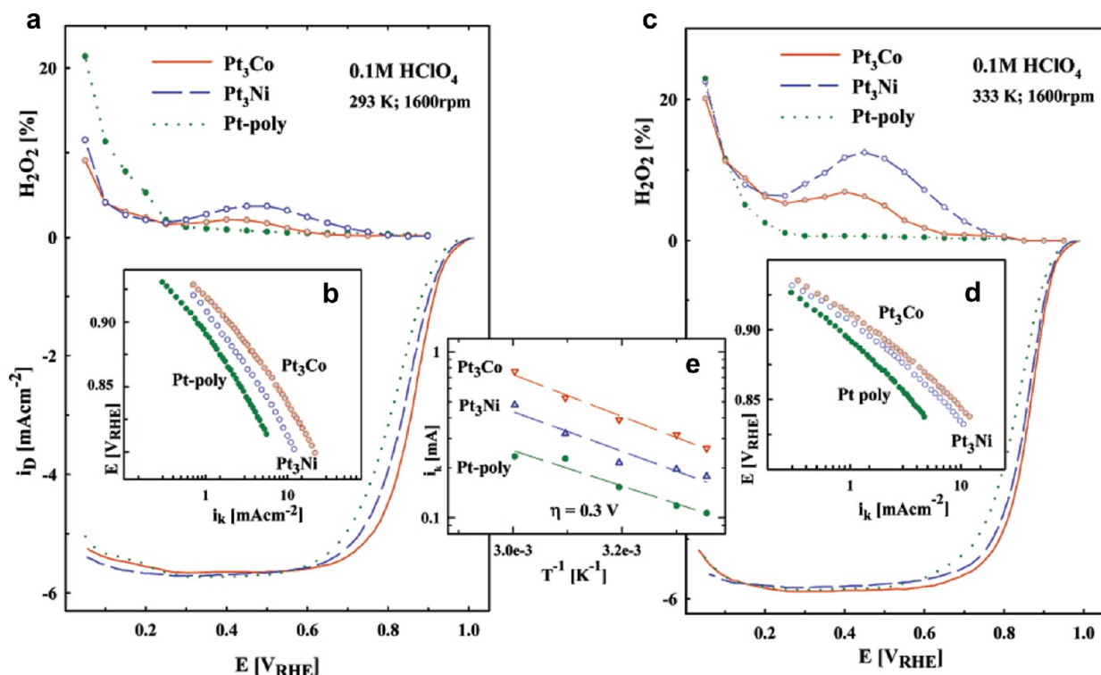
Figure 3. (a) Disk ( i_D ) and ring ( i_R ) currents (anodic sweep direction) during the ORR on mildly sputtered Pt, Pt_3Co , and Pt_3Ni in 0.1 M HClO_4 at 293 K. (b) Tafel plots for all three surfaces at 293 K. (c) Disk ( i_D ) and ring ( I_R ) currents (anodic sweep direction) during the ORR on mildly sputtered Pt, Pt_3Co , and Pt_3Ni in 0.1 M HClO_4 at 333 K. (d) Tafel plots for all three surfaces at 333 K. Conditions: sweep rate, 20 mV/s; ring potential, E = 1.15 V vs RHE; collection efficiency, N = 0.2 . (e) Arrhenius plots at an overpotential of 0.3 V for the ORR on Pt, Pt_3Co , and Pt_3Ni electrodes. Reprinted with permission from ref 40, 2002, American Chemical Society.
