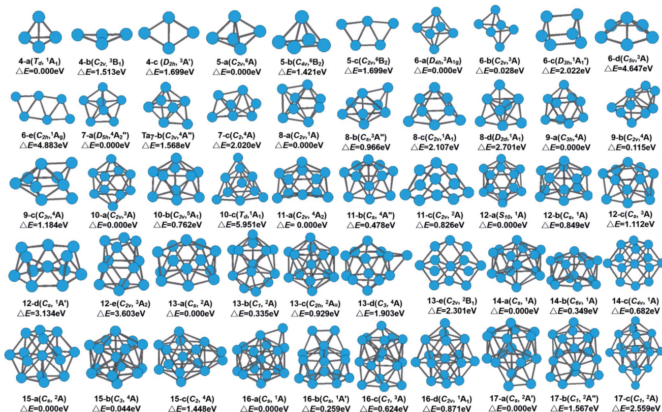
Fig. 1 Calculated stable geometries of neutral Ta_n ( n = 4-17 ) clusters.
