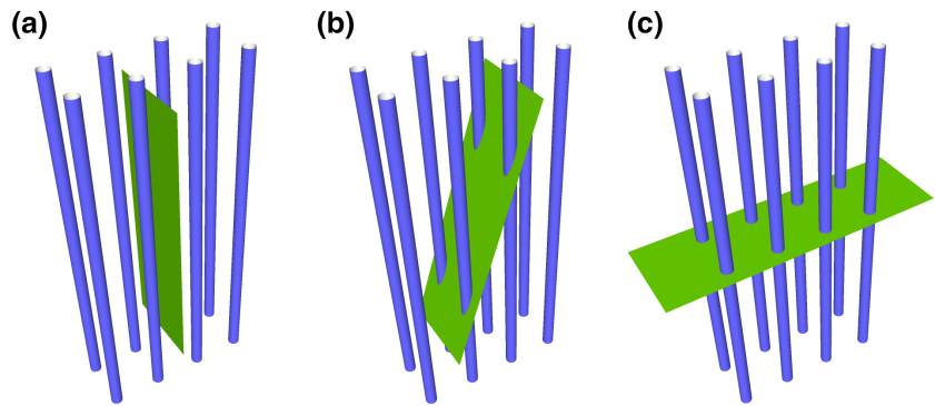
FIGURE 24 Orientation effects on interactions between a length and an area. The number of interactions between area and length is sensitive to orientation. Even though the blue length and green area are identical in all three images, 0 interactions are observed in (a), 4 in (b), and 8 in (c). This orientation sensitivity applies to estimates of length using area probes and to estimates of area using line probes [Color figure can be viewed at wileyonlinelibrary.com ]
