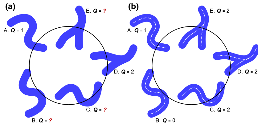
FIGURE 28 Identifying interactions of lengths with an area probe. Sometimes it is easy to decide how many interactions need to be counted based on the appearance of the objects of interest alone (Objects A and D in (a)). Other objects are more doubtful (B, C, and E in (a)). If one does not want to count touches as interactions between the spaceball and the length that is to be estimated, imagining the spines (white broken lines in (b)) may be helpful. Even though object C touches the circle only once, the spine of this object crosses the spaceball twice. We need to count two interactions. Instead, object B touches the spaceball twice, but its spine does not intersect the surface of the spaceball. No interactions are counted. Even though object E interacts only once with the surface of the spaceball, its spine crosses twice and two interactions need to be counted [Color figure can be viewed at wileyonlinelibrary.com ]
