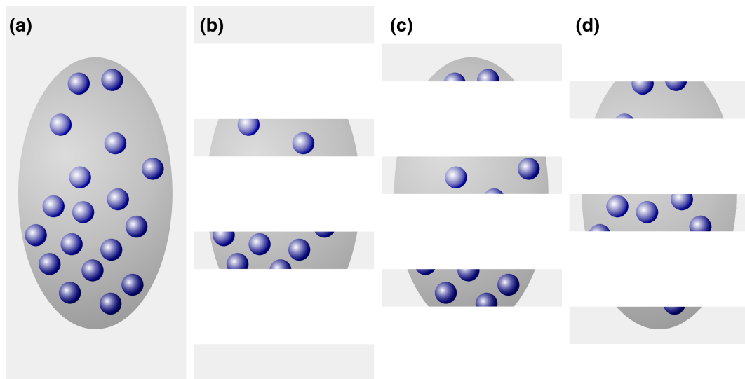
FIGURE 2 Profile counts cannot be extrapolated to total cell number. (a) A region (dark gray) containing 18 cells (blue objects) is cut into three series of sections (b–d). In each series, the profiles of cells visible in the sections are counted. Eight cell profiles are counted in the two sections of the region contained in series (b). The three sections in series (c) contain 10 cell profiles. The three sections in series (d) contain nine cell profiles. Extrapolating the mean profile count, 9, to total cell number by multiplying with 3 generates an estimate of 27 cells instead of the true value of 18 cells [Color figure can be viewed at wileyonlinelibrary.com ]
