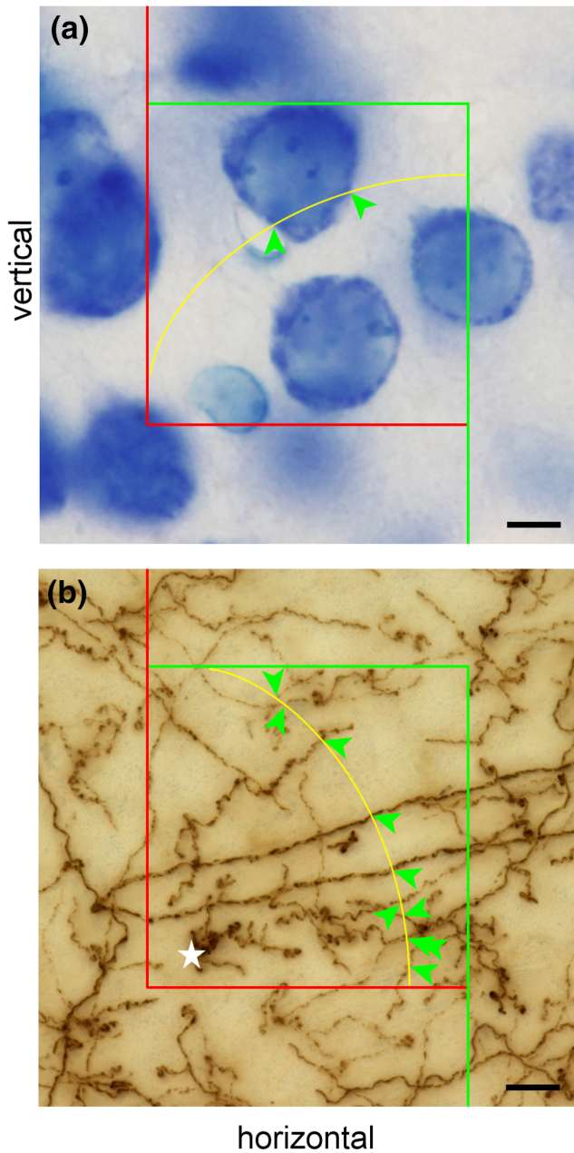
FIGURE 35 Surface and length estimates in vertical sections. (a) A cycloid line probe intersects twice with the surface of a neuron. Scale bar: 5 \mu\text{m} . (b) A cycloid area probe intersects 10 times with tyrosine hydroxylase immunoreactive axons in a minimum density projection of an image stack spanning a 40 \mu\text{m} thick section. Image planes were spaced 0.2 \mu\text{m} apart. To resolve interactions between an area probe and axons in dense axon clusters (asterisk), the image stack would have to be examined image by image. Scale bar: 10 \mu\text{m} [Color figure can be viewed at wileyonlinelibrary.com ]
