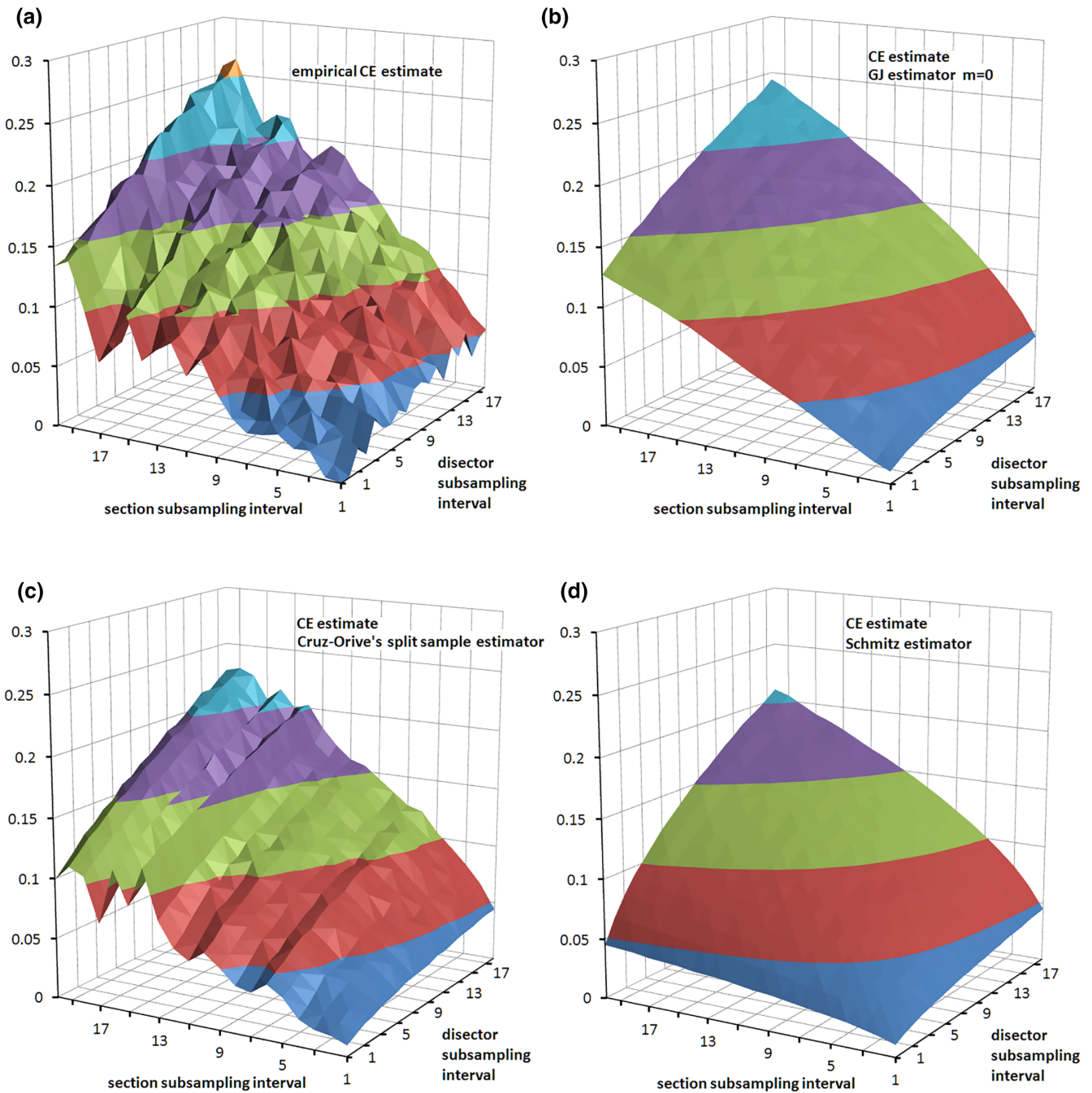
FIGURE 40 Empirical CE estimates and CE estimators. In (a), CEs of a number estimate were estimated empirically by collecting a very large data set from hippocampal CA1 pyramidal cells (Sloianka & West, 2005). From this data set subsamples were drawn and the CEs were estimated (CV of the mean of all subsamples for each combination of subsampling intervals). The Gundersen–Jensen (GJ) estimator (b) and Cruz–Orive’s split sample estimator (c) provide useful approximations of the variance generated by the sampling. The estimator of Schmitz (1998) (d) considers only the variance component generated by sampling within sections and provides a simple to calculate, rough-and-ready estimate if the sampling of sections contributes very little variance to estimates [Color figure can be viewed at wileyonlinelibrary.com ]
