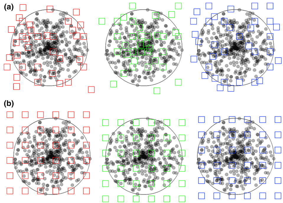
FIGURE 7 Uniform random independent sampling and uniform random systematic sampling. The area of a section containing unevenly distributed objects is probed in (a) with three uniform random independent samples of the area (red, green, and blue squares) and in (b) with three uniform random systematic samples of the area. Both types of sampling are statistically representative. However, note that the systematic samples, unlike the blue independent sample, never completely miss the central part of the section, in which the objects of interest are spaced closely together. Also, they never, like the green independent sample, contain an unduly large number of samples in the central part of the section [Color figure can be viewed at wileyonlinelibrary.com ]
