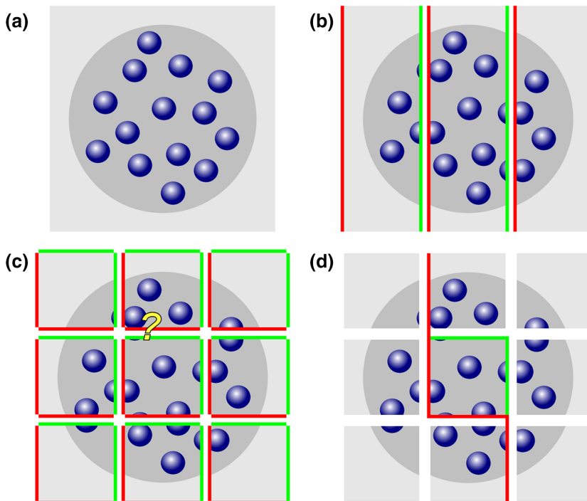
FIGURE 17 The unbiased counting frame. A section containing 14 objects (a) is successively divided first parallel to the y-axis (b) and then parallel to the x-axis (c). Along the dividing lines, the same counting rules that have been established along the z-axis are now applied along the x- (b) and then x- and y-axes (d). Fifteen objects instead of 14 are detected if all objects fully contained within the squares and all object fragments touching a green inclusion line are counted in (c). The overcount is due to the double count of the cell labeled with the question mark. The double count is avoided by the extension of the red exclusion lines in (d) [Color figure can be viewed at wileyonlinelibrary.com ]
