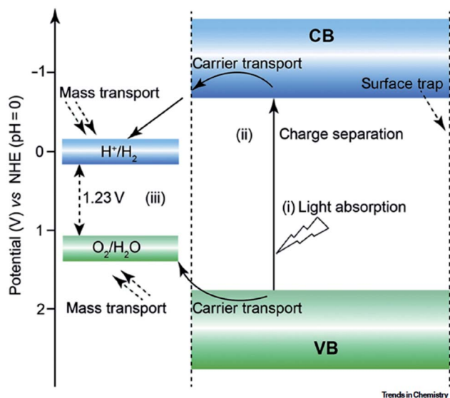
Fig. 12 Basic mechanism for the photocatalytic hydrogen production. This figure has been adapted from ref. 90 with permission from CELL PRESS, copyright 2020.
