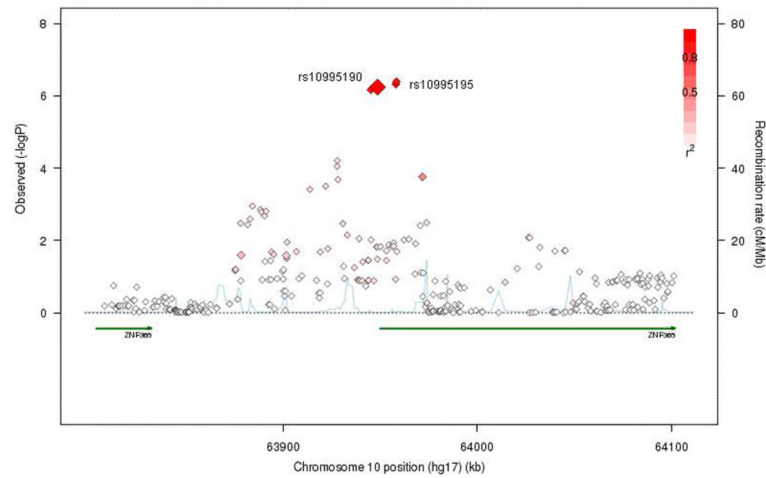
Figure 1. Regional association plot for ZNF365 across a 300kb window. Association of individual SNPs is plotted as -\log_{10}(P) against chromosomal base-pair position. Results of both genotyped and imputed SNPs are provided. Colors indicate the LD relationship between rs10995190 and the other markers (red, r^2 > 0.8 ). The right-hand Y axis shows the recombination rate estimated from the HapMap CEU population. All p-values are from the discovery phase.
