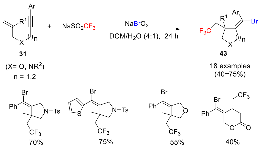
Scheme 38. \text{NaSO}_2\text{CF}_3 / \text{NaBrO}_3 -promoted bromotrifluoromethylation of enynes.
