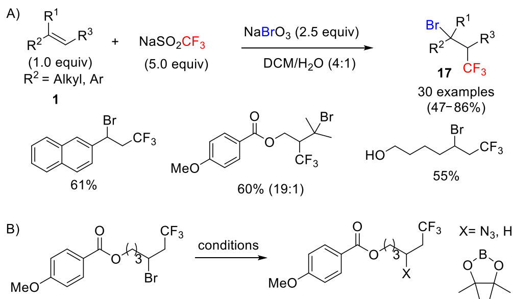
Scheme 36. NaBrO 3 -promoted bromotrifluoromethylation of styrenes and unactivated alkenes (A); utility of the obtained product 17 (B).
