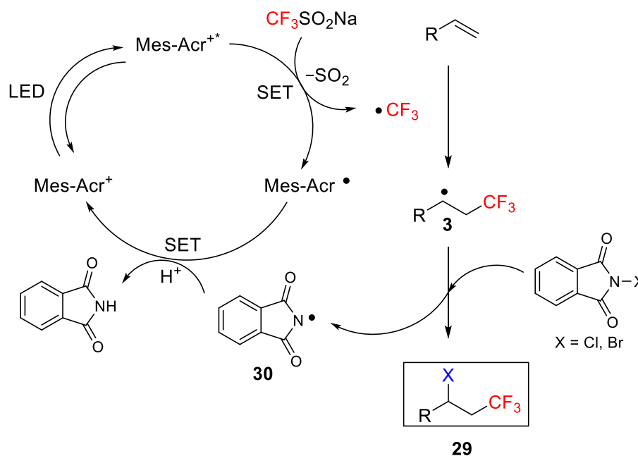
Scheme 22. Proposed mechanism for the halotrifluoromethylation of alkenes.
