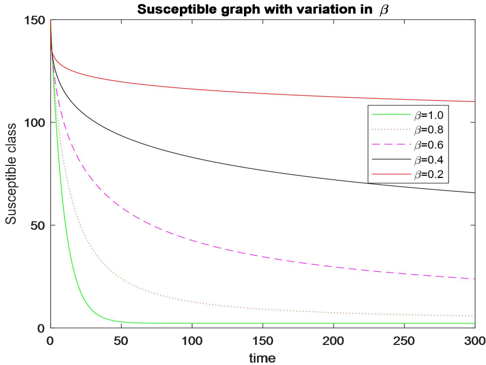
Figure 1: Graphical illustration of the susceptible class showing different values of \beta .
