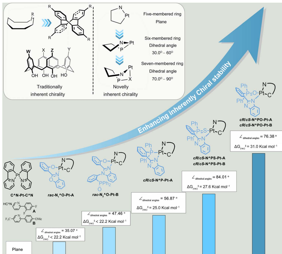
Fig. 1 The designed scheme and chemical structures of inherently chiral Pt(II) complexes ( \angle dihedral angles: angle between the phenyl plane and the PtC N coordination plane; \Delta G_{rac}^{\ddagger} : racemization energy barriers of inherently chiral Pt(II) complexes).
