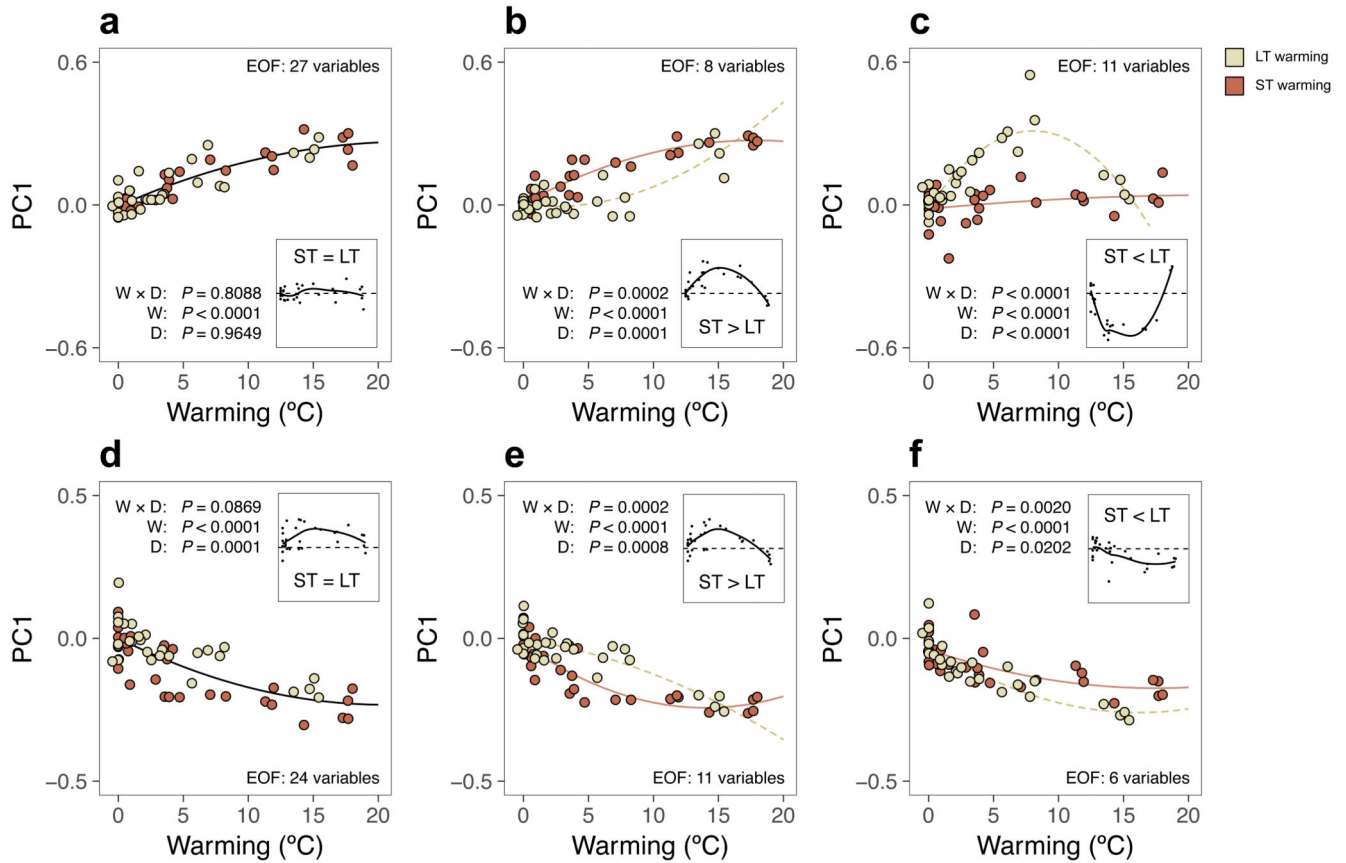
Figure 2. Response shapes under soil warming.
