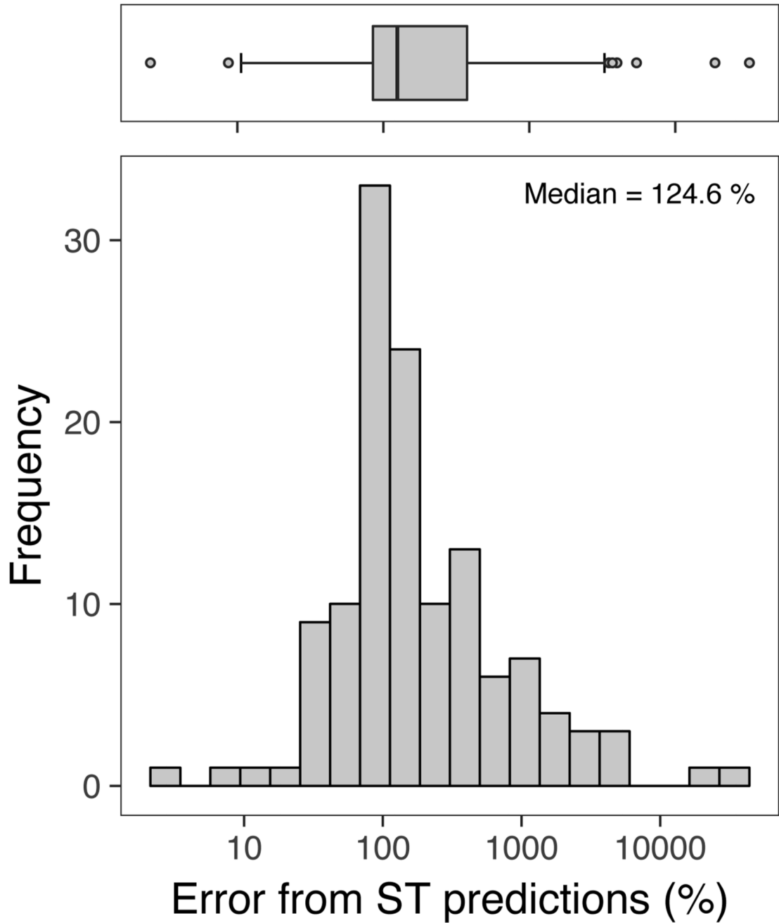
Figure 4. Prediction errors from short-term observations.
