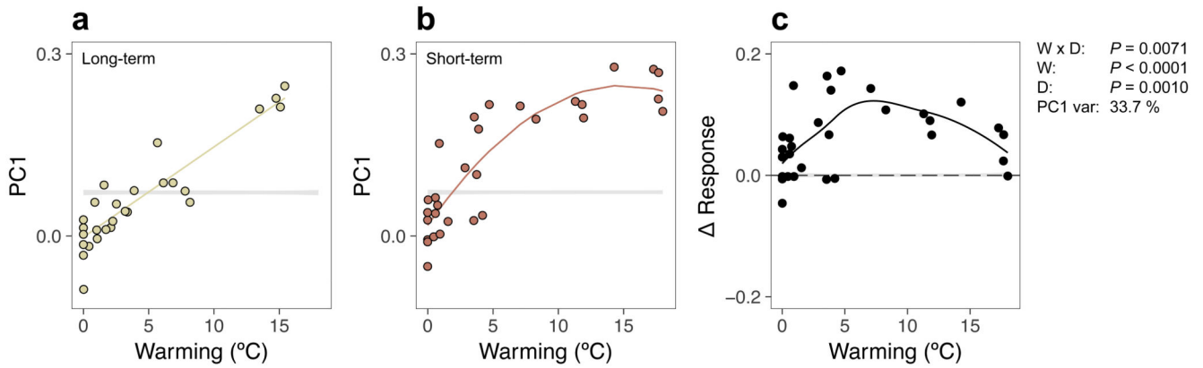
Figure 1. Whole-ecosystem responses to soil warming.
