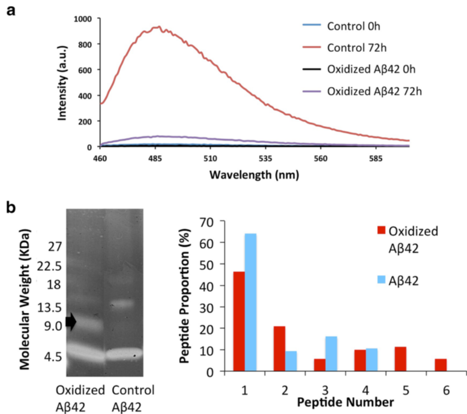
Figure 3 Thioflavine T fluorescence and SDS PAGE of oxidized and control A \beta 42. a) ThT fluorescence spectra following fibril formation from A \beta 42 (20 \mu M) in the presence or absence of Cu 2+ and H 2 O 2 for 72 hours. The spectra for oxidized and control samples show an increased intensity over the incubation time and show increased ThT signal for non-oxidized compared to oxidized samples. b) SDS PAGE showing separation of A \beta 42. Oxidized A \beta 42 (left column) runs as monomer and dimer (approx. 9 kDa, black arrow), whilst non oxidized, control A \beta 42 (right column) shows bands corresponding to monomer and trimer as previously observed [44]. The trimer is thought to be induced by SDS [44]. Densitometry confirms that monomer is the strongest band following by dimer for oxidized but not control fibrils. This reveals that the dimer is enriched under oxidation conditions.
