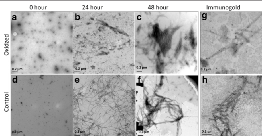
Figure 4 Transmission electron microscopy images of freshly formed A \beta 42 fibrils. 20 \mu M A \beta 42 (pH 7.4) was incubated in the presence of Cu 2+ /H 2 O 2 ( a, b, c ) and compared to 20 \mu M A \beta 42 in phosphate buffer alone (pH 7.4) ( d, e, f ). Assembly was monitored by electron microscopy after incubation for (a and d) zero hours, (b and e) 24 hours and (c and f) 48 hours. Both oxidized and control A \beta 42 samples show oligomeric species at zero hour ( a, d ) and fibrils following 48 hour incubation ( c, g ). However, at 24 hours (b and f) fibrils were observed in non-oxidized conditions ( f ), but no fibrils were observed in oxidised conditions ( b ). The presence of dityrosine was detected using immunogold labeling using a dityrosine specific antibody that labeled oxidized fibrils ( g ) but not control fibrils ( h ).
