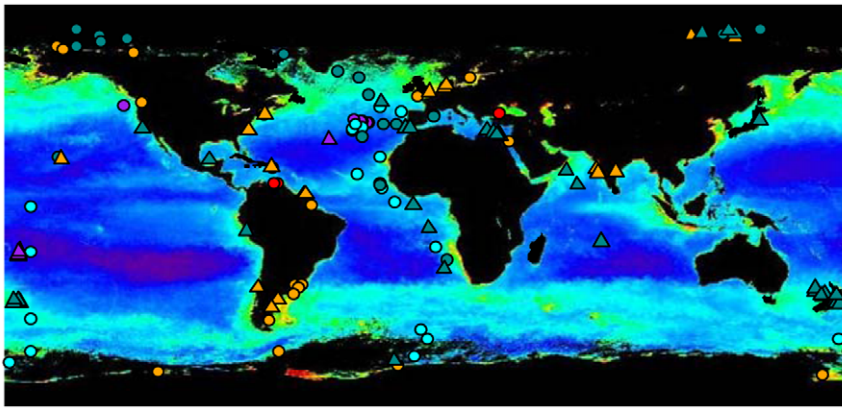
Figure 1. Global map of sample locations. Sample locations were plotted on a SeaWiFS satellite image of chlorophyll pigment concentration, with redder colour representing higher concentrations. The realm origin of the samples is indicated by circles (pelagic) and triangles (benthic), whereas ecosystem types are indicated by the colour orange (coastal), light blue (open ocean surface waters), dark blue (deep-sea), red (anoxic), and purple (hydrothermal vents). Further visualization of sample distribution e.g. on a bathymetric map is available at http://vamps.mbl.edu/mapper/index.php .
