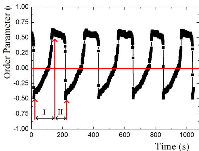
Figure 7 | Relative height difference \phi , as an order parameter exhibits an excellent periodicity in the APS pattern at P = 50 kPa and \Gamma = 6.2 . The procedure (I) corresponds to the percolation stage, and (II) corresponds to the eruption stage.
