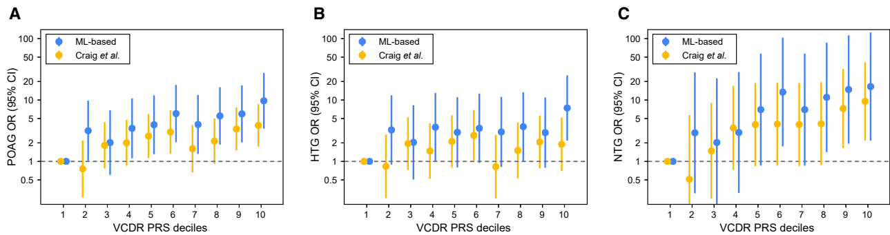
Figure 5. Primary open-angle glaucoma (POAG) prediction in the EPIC-Norfolk cohort
