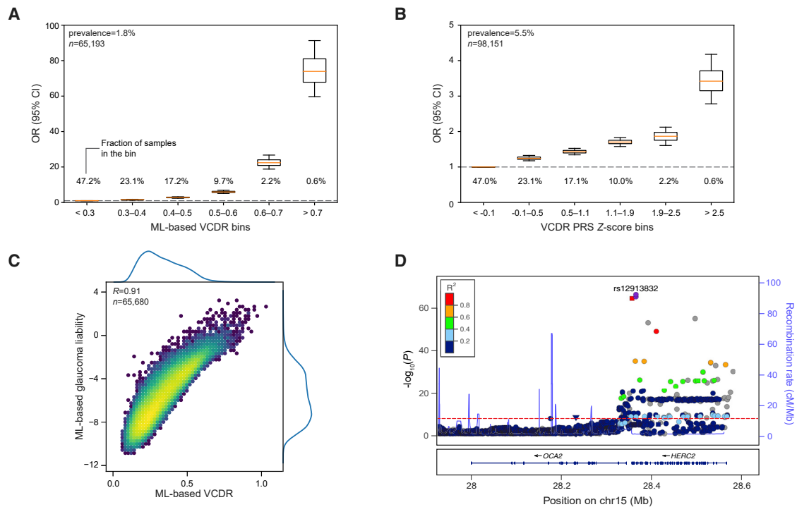
Figure 4. Relationship between glaucoma and VCDR
