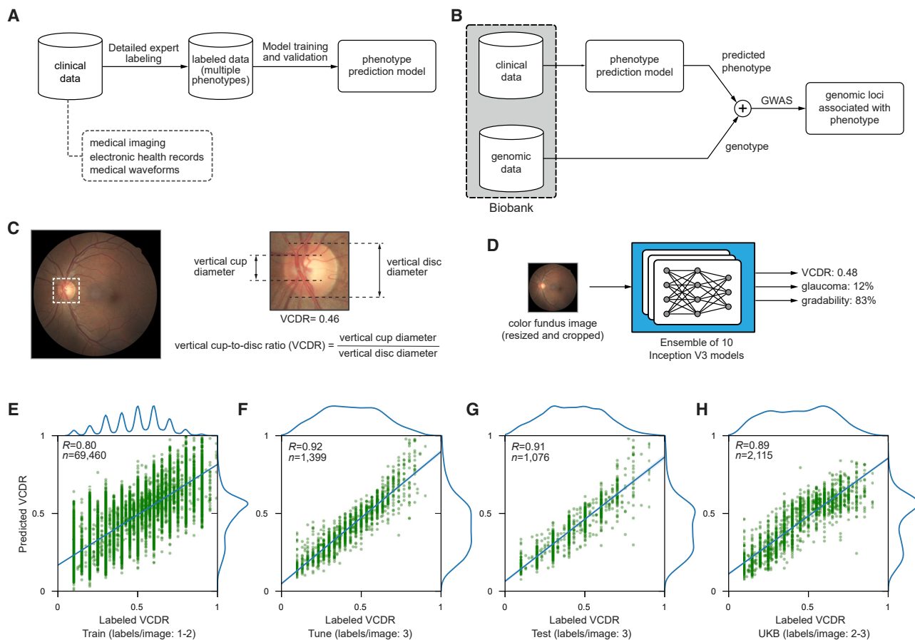
Figure 1. ML-based phenotyping concept and its application to VCDR
