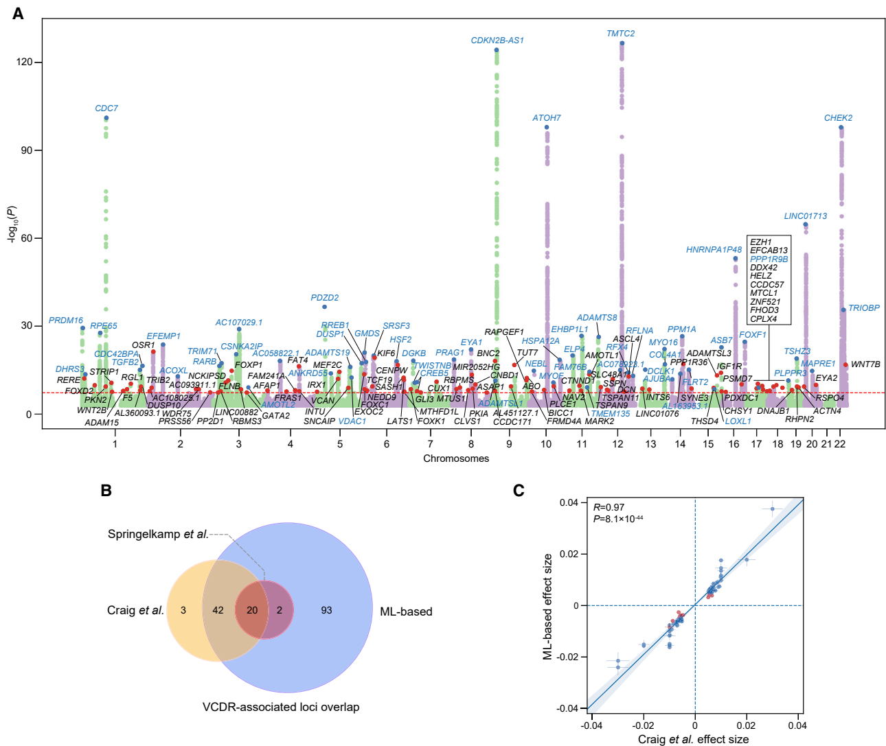
Figure 2. ML-based VCDR GWAS results and comparison to known associations
