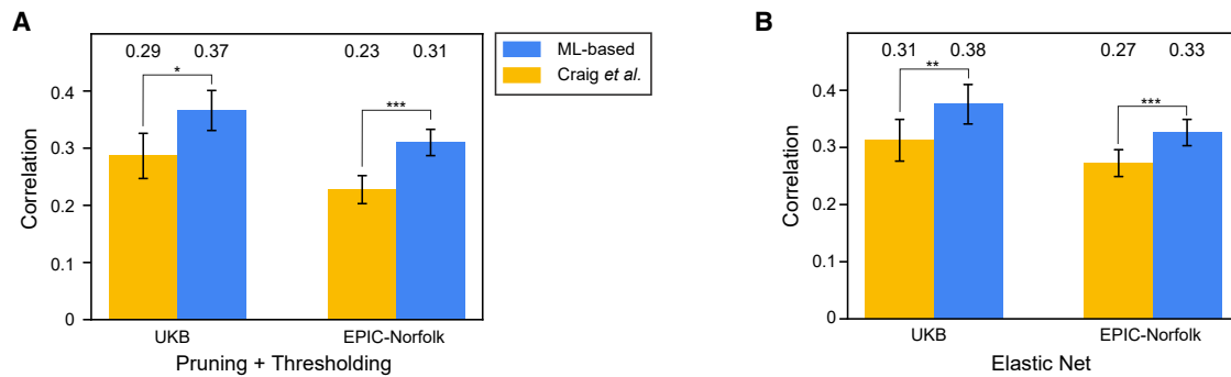
Figure 3. VCDR polygenic risk score performance metrics
