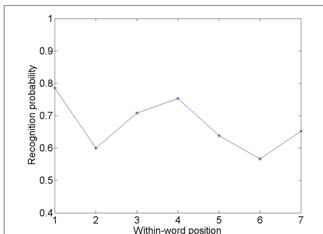
FIGURE 2 | Letter visibility (recognition probability) as a function of within-string position, for a seven-letter string with fixation on the central position (i.e., the fourth letter) from Stevens and Grainger, 2003. Note that this recognition curve is based on data collected in French.
