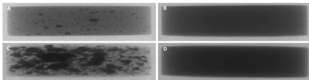
Fig 7. Transverse view of X \mu CT reconstruction of placebo tablets (13mm) containing contrast material in the core. Contrast material Bi 2 O 3 is included at 5% w/w and 10% w/w (milled), A and B respectively. BaSO 4 is included at 10% w/w and 20% w/w (milled), C and D respectively.
